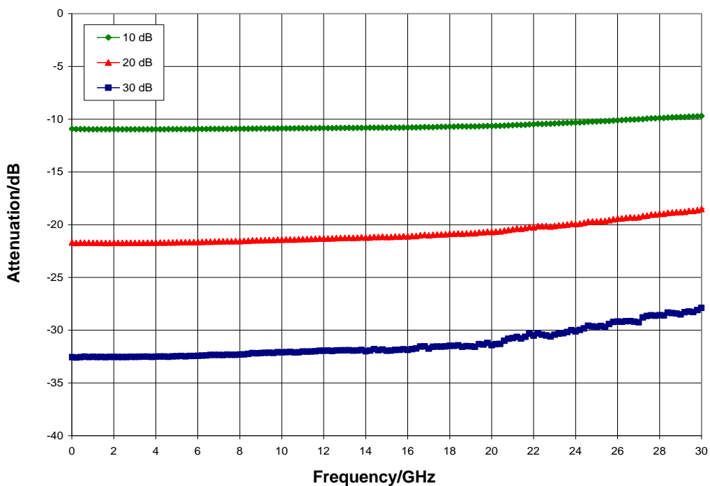
Normalized Attenuation (all states), T_A = 25^\circ\text{C}
