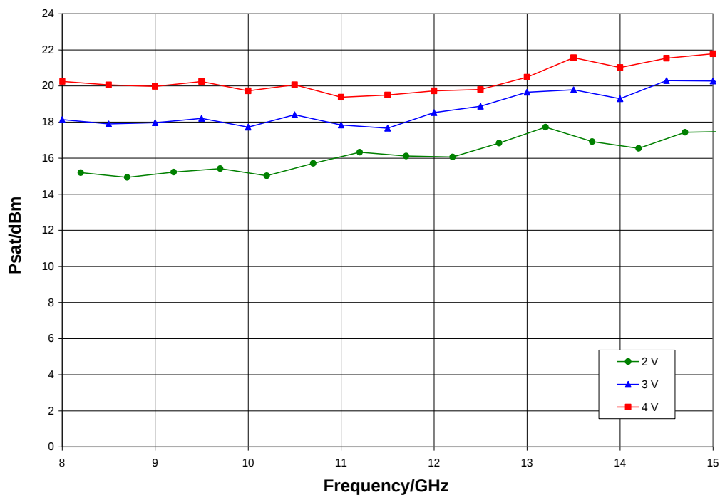
Psat vs. V_{dd} , V_{gg} = 1.5\text{ V} , T_A = 25^\circ\text{C}
