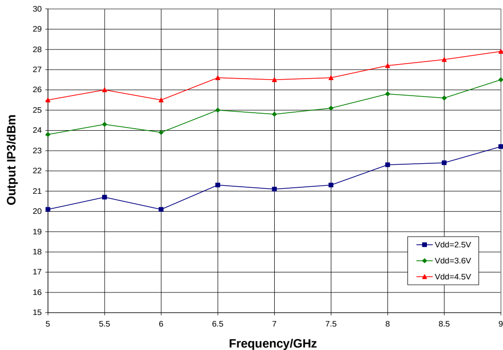
Output IP3 vs. V_{dd} , T_A = 25\text{ °C}
