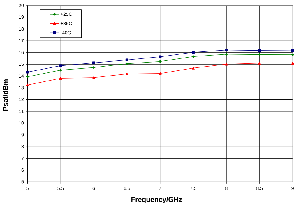
Psat vs. Temperature, V_{dd} = 3.6\text{ V}
