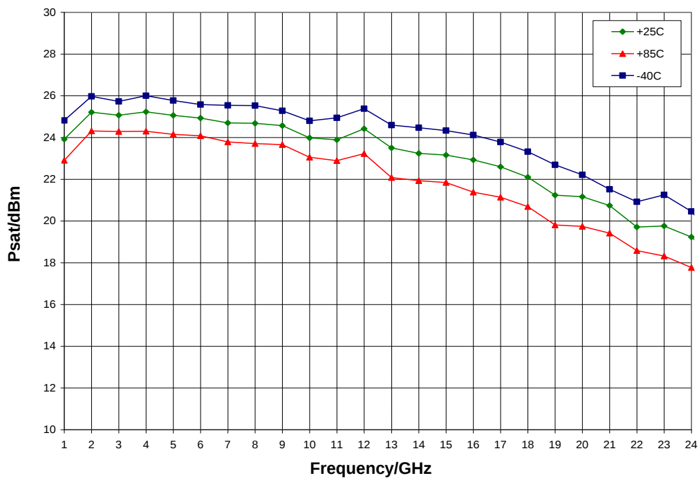
Psat vs. Temperature, V_{dd} = 8.0\text{ V}
