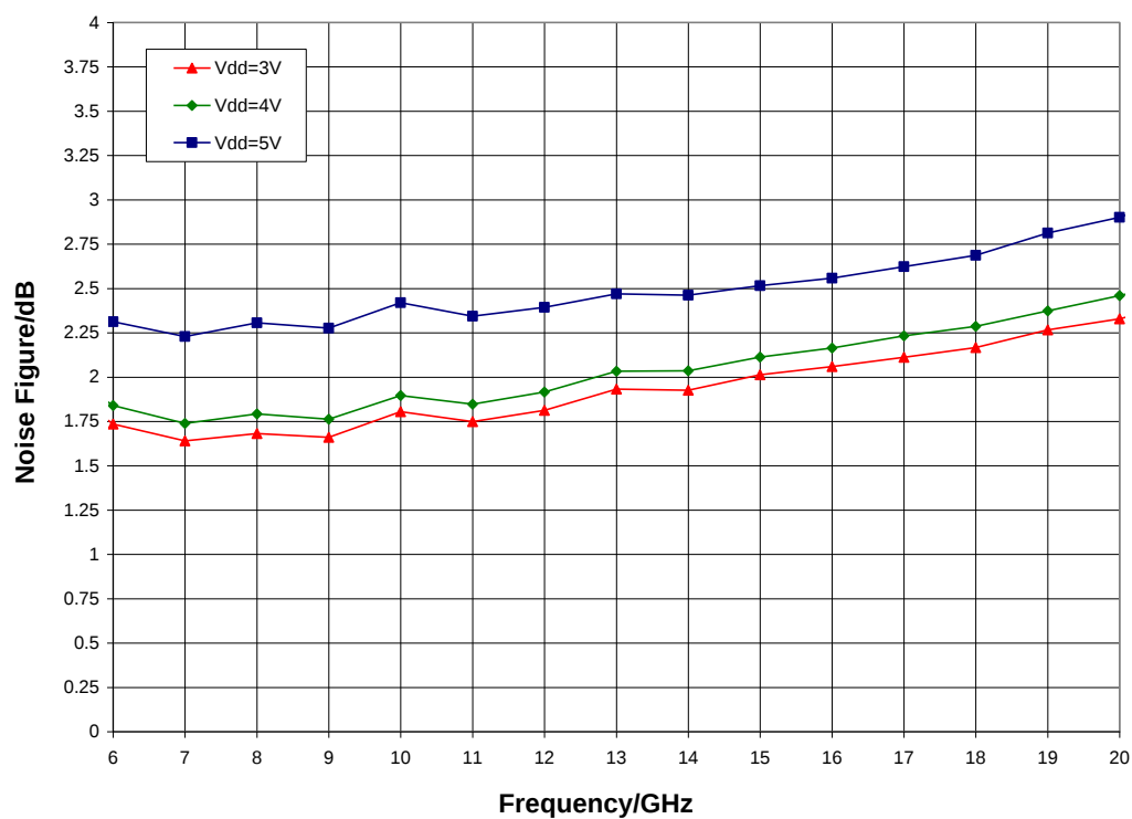
Noise Figure vs. V_{dd} , T_A = 25^\circ \text{C}
