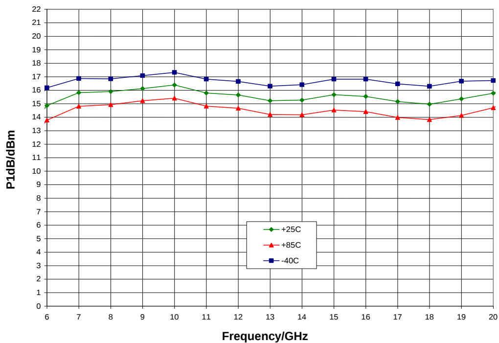
P1dB vs. Temperature, V_{dd} = 4.0\text{ V}
