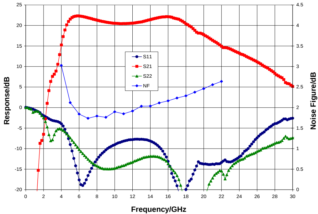
Broadband Performance, V_{dd} = 4.0 V, T_A = 25 °C
