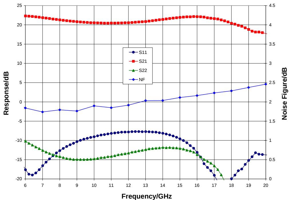
Narrow-band Performance, V_{dd} = 4.0 V, T_A = 25 °C
