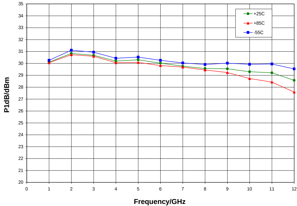
P1dB vs. Temperature, V_{dd} = 12.0 V, V_{gg1} = -0.16 V, V_{gg2} = 4.75 V, I_{dd} = 450 mA, T_A = 25^\circ C
