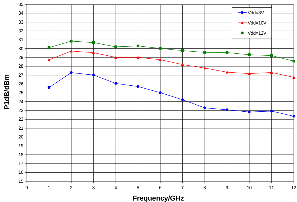
P1dB vs. Supply Voltage, V_{gg1} = -0.16 V, V_{gg2} = 4.75 V, I_{dd} = 450 mA, T_A = 25^\circ C
