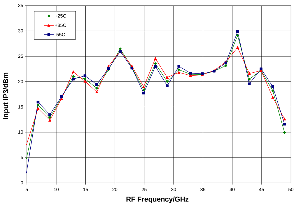
Input IP3 vs. Temperature, LO = +19 dBm, IF = 900 MHz USB
