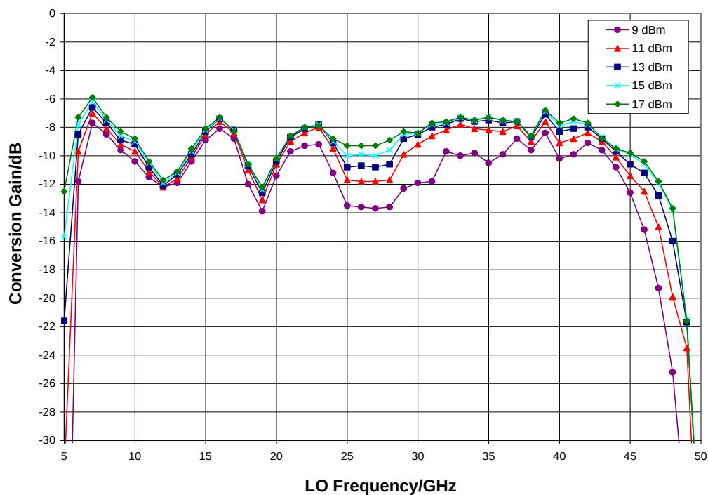
Conversion Gain vs. LO Drive, IF = 900 MHz USB
