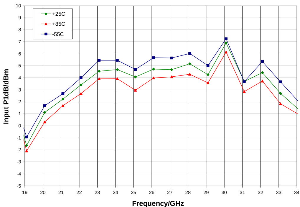
Input P1dB vs. Temperature, LO = -4 dBm, T_A = 25^\circ\text{C}
