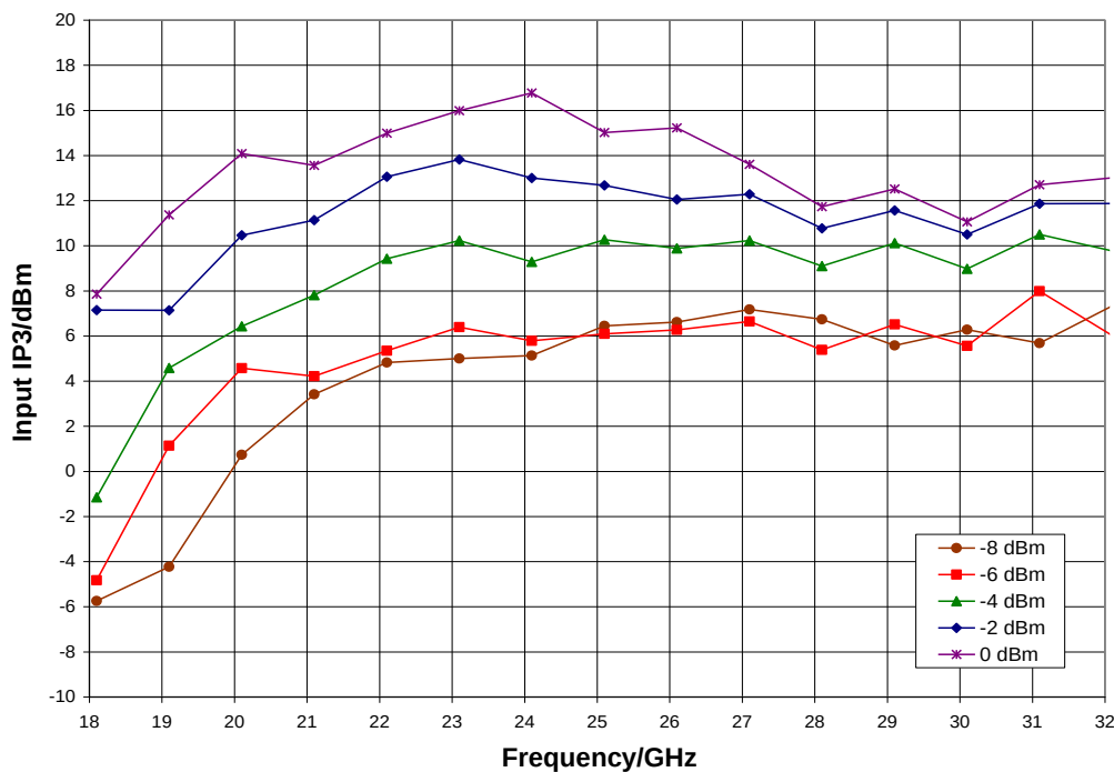
Input IP3 vs. LO Drive, T_A = 25^\circ\text{C}
