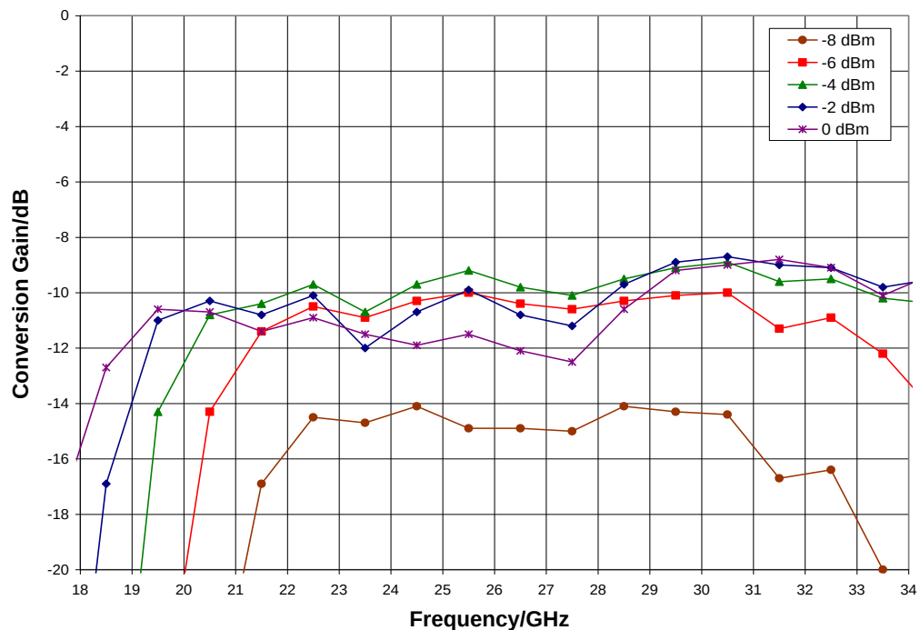
Upconverter Performance, Conversion Gain vs. LO Drive, T_A = 25^\circ\text{C}
