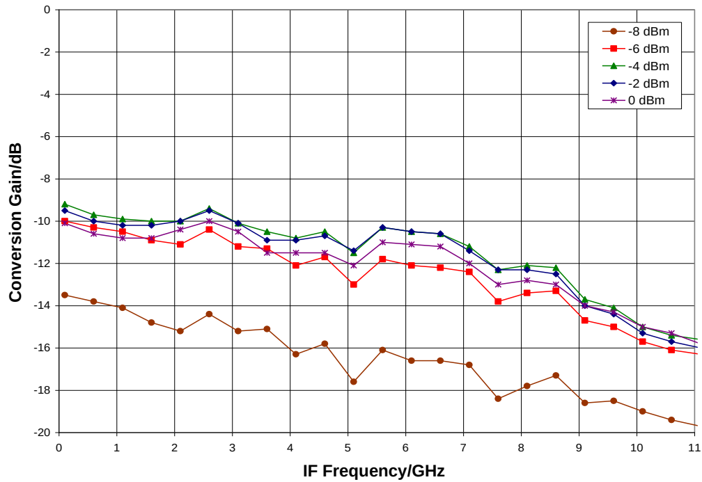
IF Bandwidth, LO = -4 dBm, T_A = 25^\circ\text{C}
