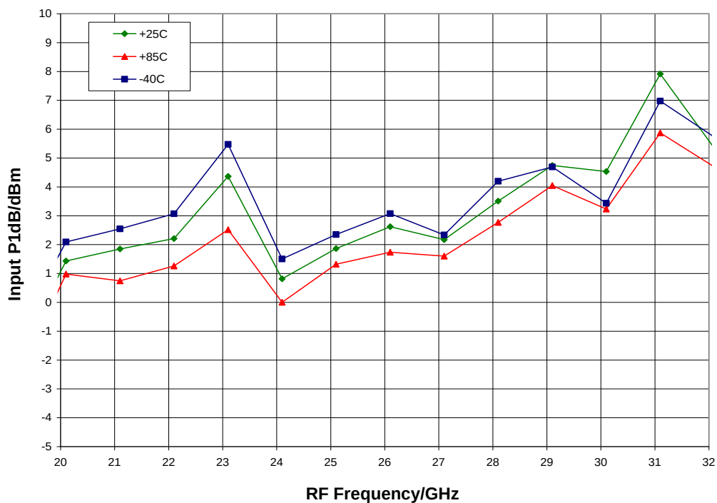
Input P1dB vs. Temperature, LO = -2 dBm, T_A = 25^\circ\text{C}
