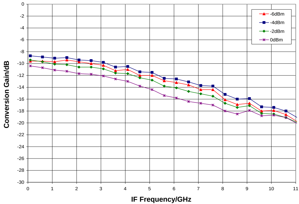
IF Bandwidth vs. LO Drive, T_A = 25^\circ\text{C}
