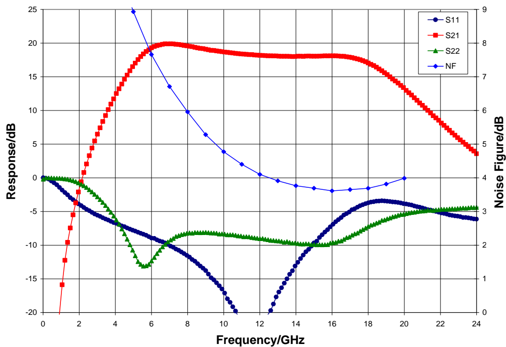
Broadband Performance, V_{dd} = 5.0\text{ V} , T_A = 25^\circ\text{C}
