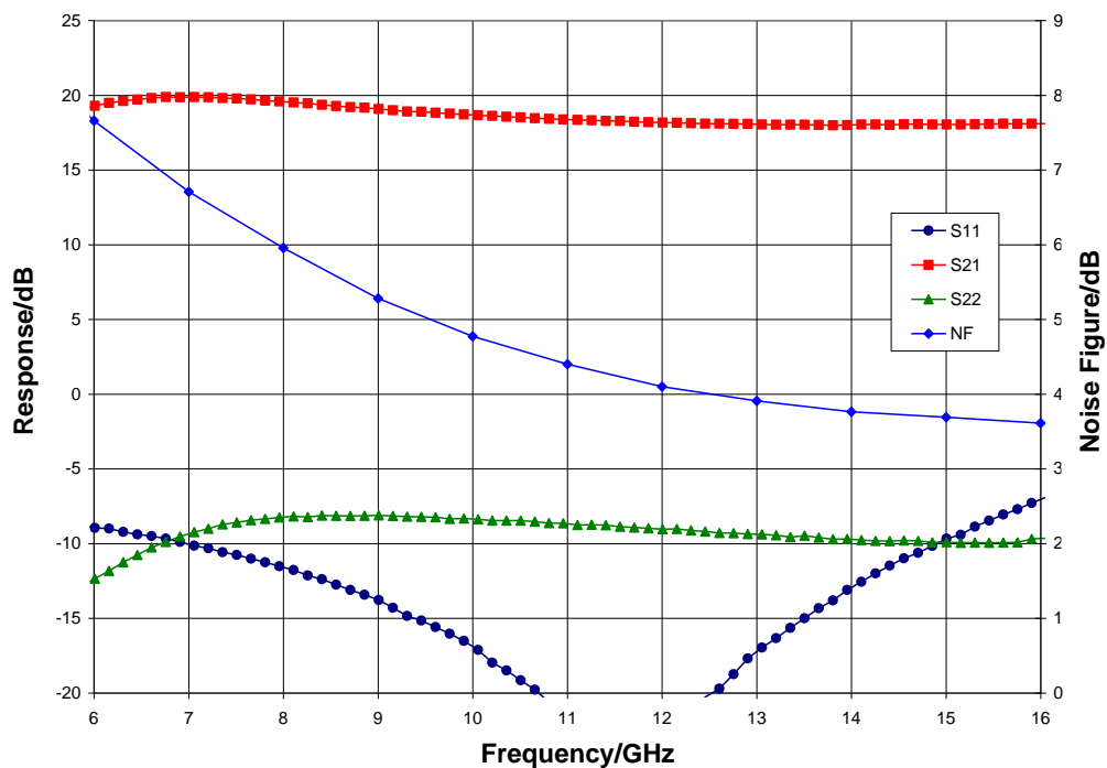
Narrow-band Performance, V_{dd} = 5.0\text{ V} , T_A = 25^\circ\text{C}
