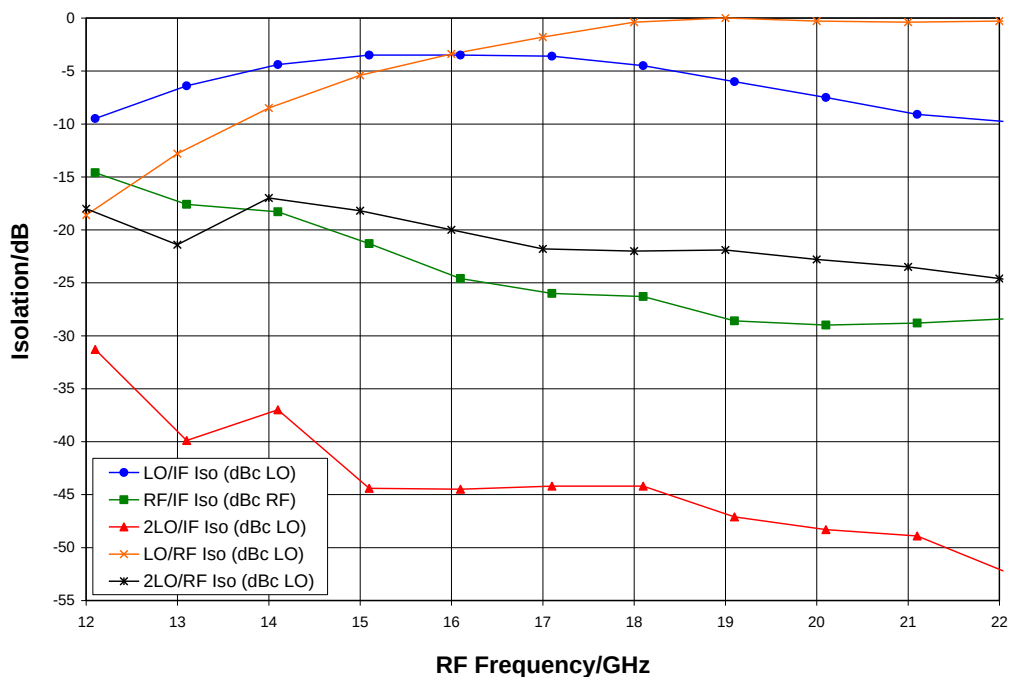
Isolations, LO = +2 dBm, RF = -10 dBm, T_A = 25^\circ\text{C}
