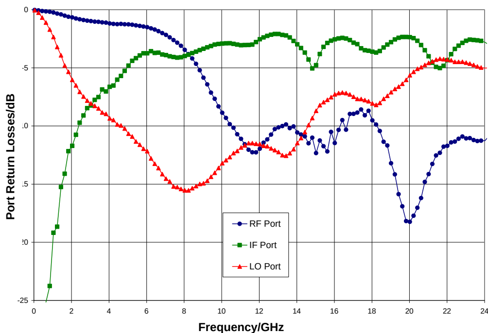
Return Loss, LO = +2 dBm, T_A = 25^\circ\text{C}
