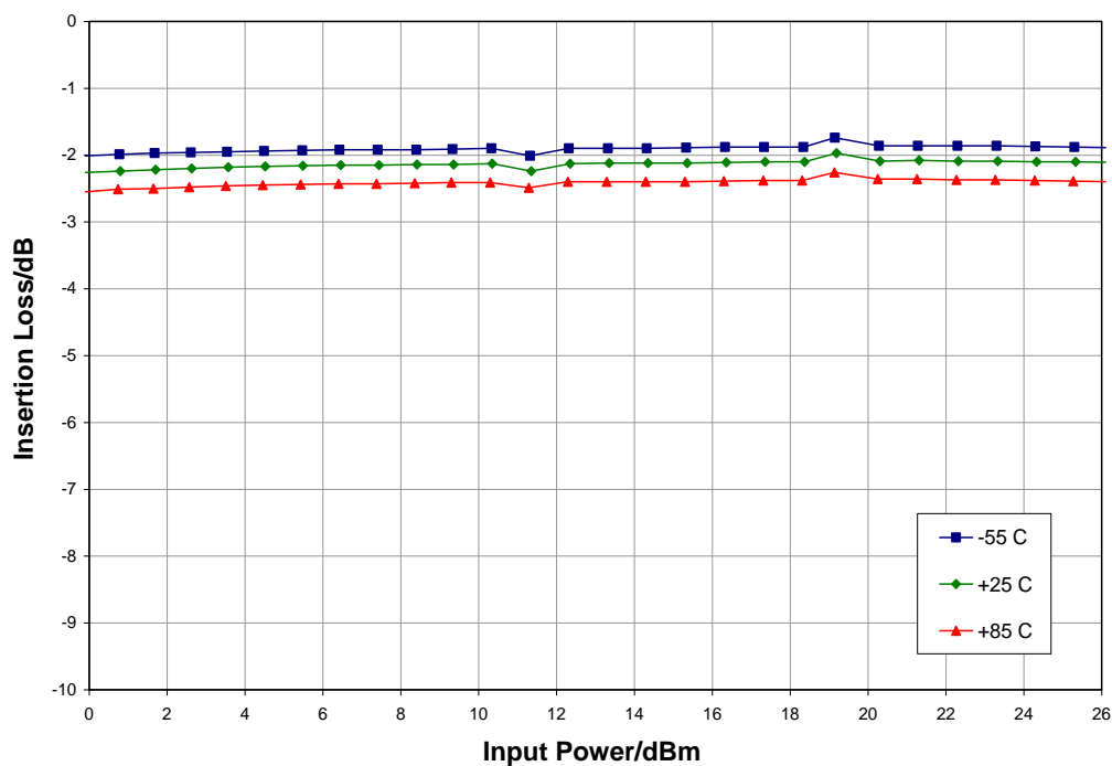
Insertion Loss vs. Pin @ 18 GHz, V_{ctl} = 0 V
