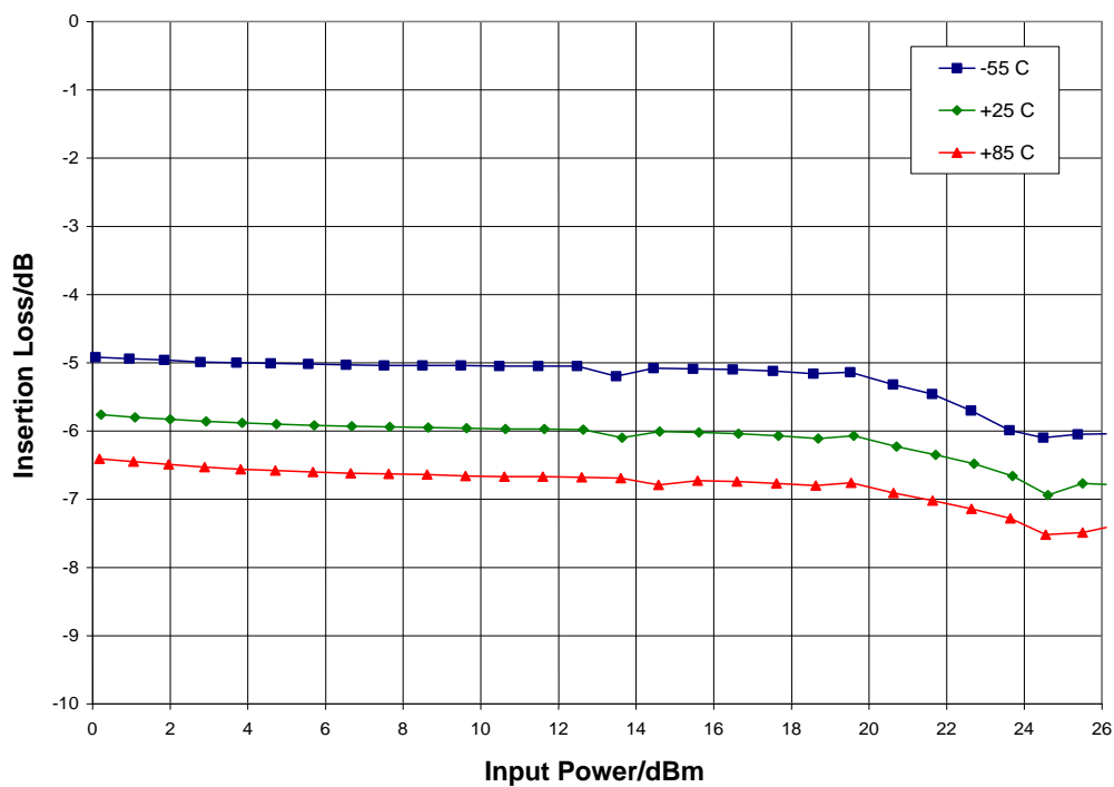
Insertion Loss vs. Pin @ 7 GHz, V_{ctl} = 0 V
