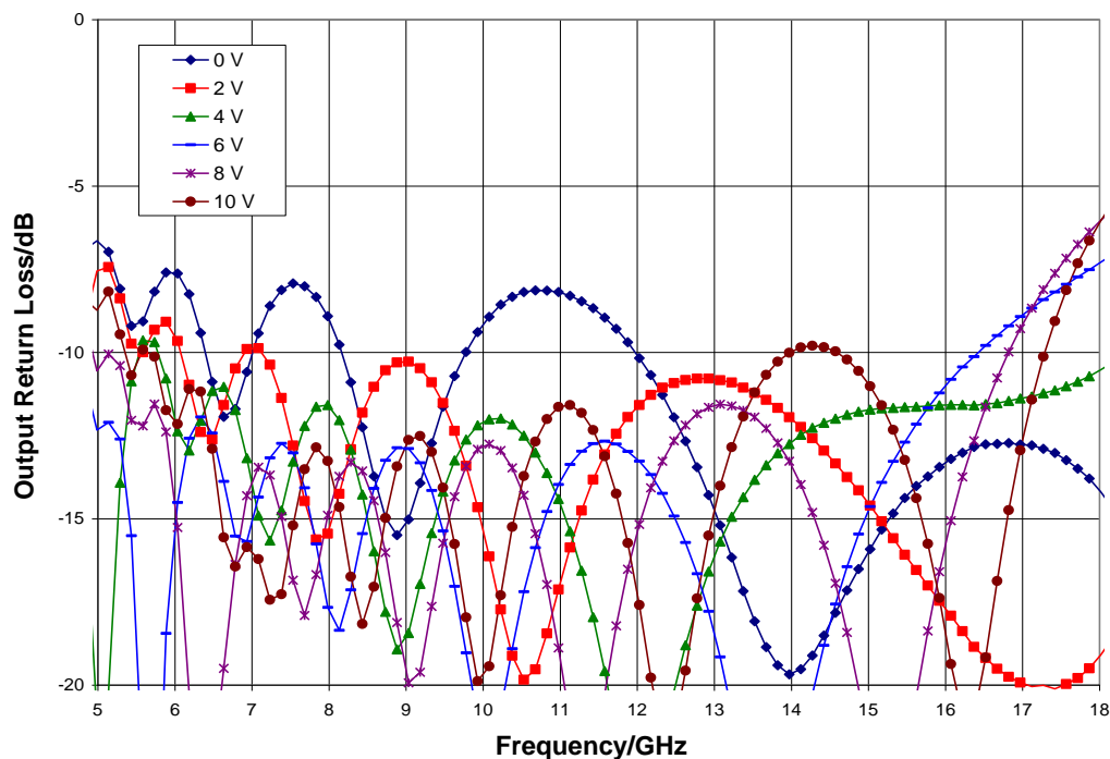
Output Return Loss, T_A = 25^\circ\text{C}
