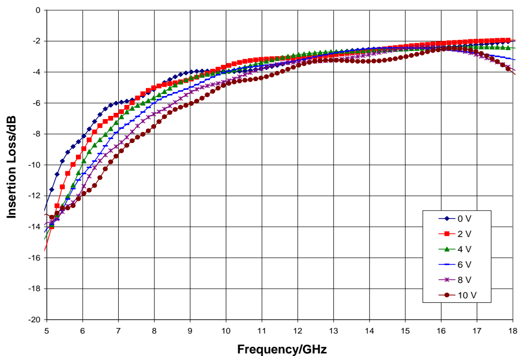
Insertion Loss vs. Frequency, T_A = 25^\circ C
