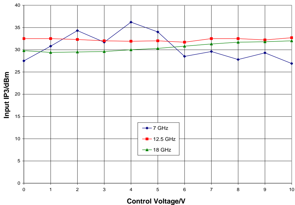
Input IP3 vs. Control Voltage, T_A = 25^\circ\text{C}
