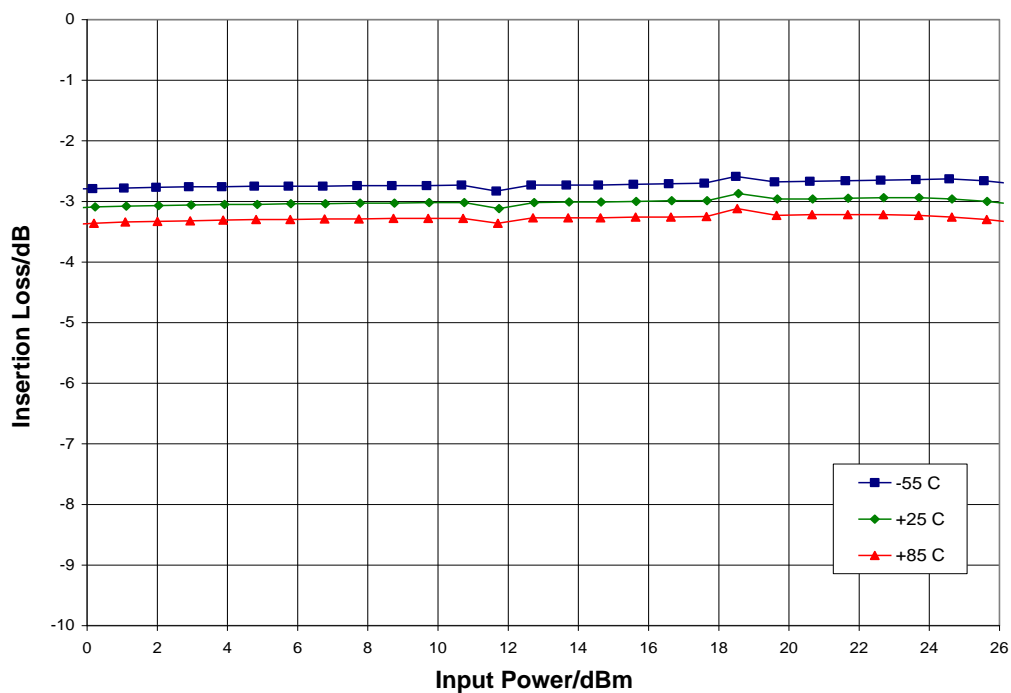
Insertion Loss vs. Pin @ 12 GHz, V_{ctl} = 0 V
