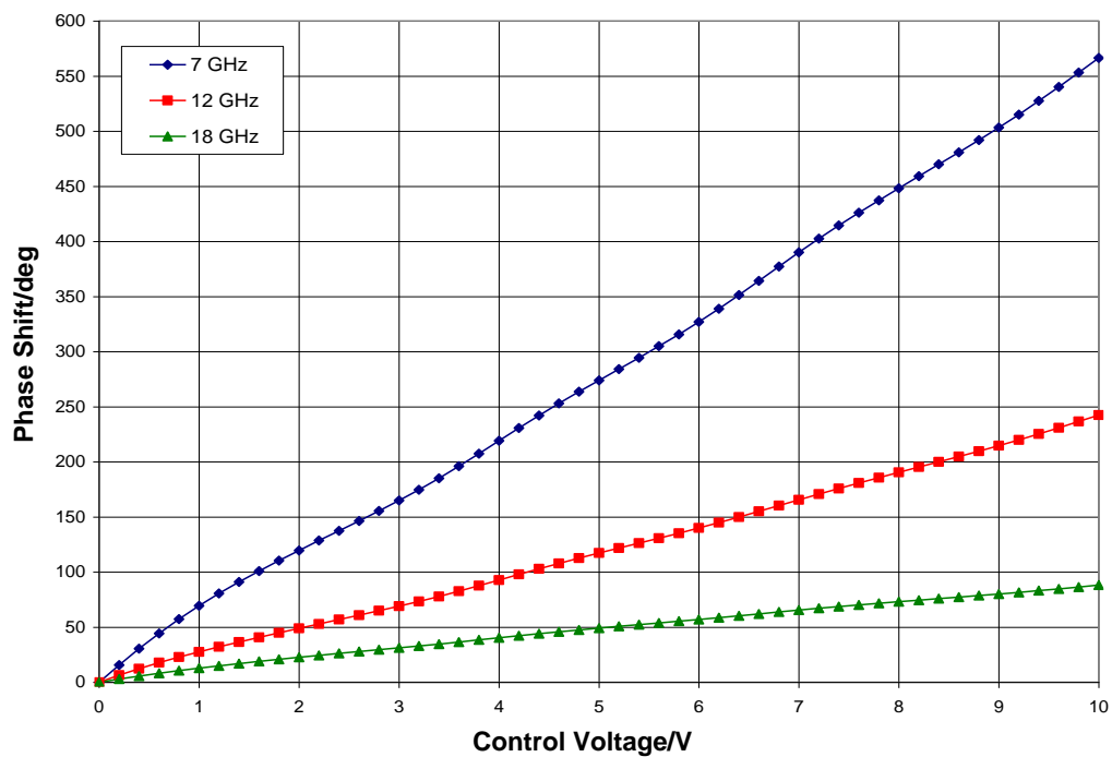
Phase Shift vs. Control Voltage, T_A = 25^\circ\text{C}
