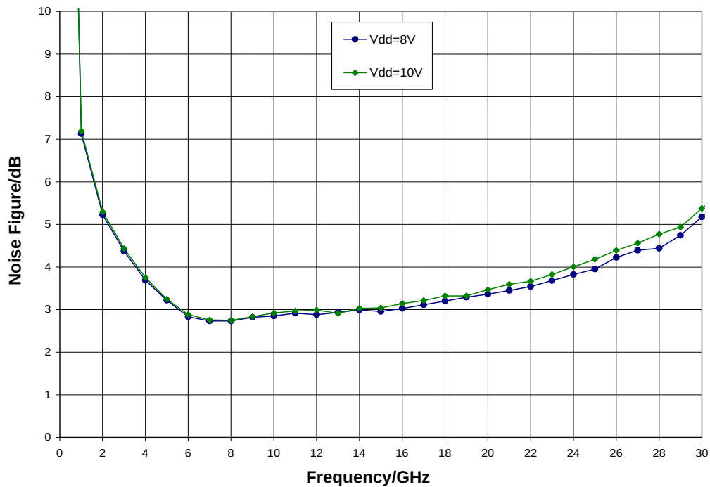
Noise Figure vs. V_{dd} , V_{gg2} = 3.5\text{ V} , I_{dd} = 250\text{ mA} , T_A = 25^\circ\text{ C}
