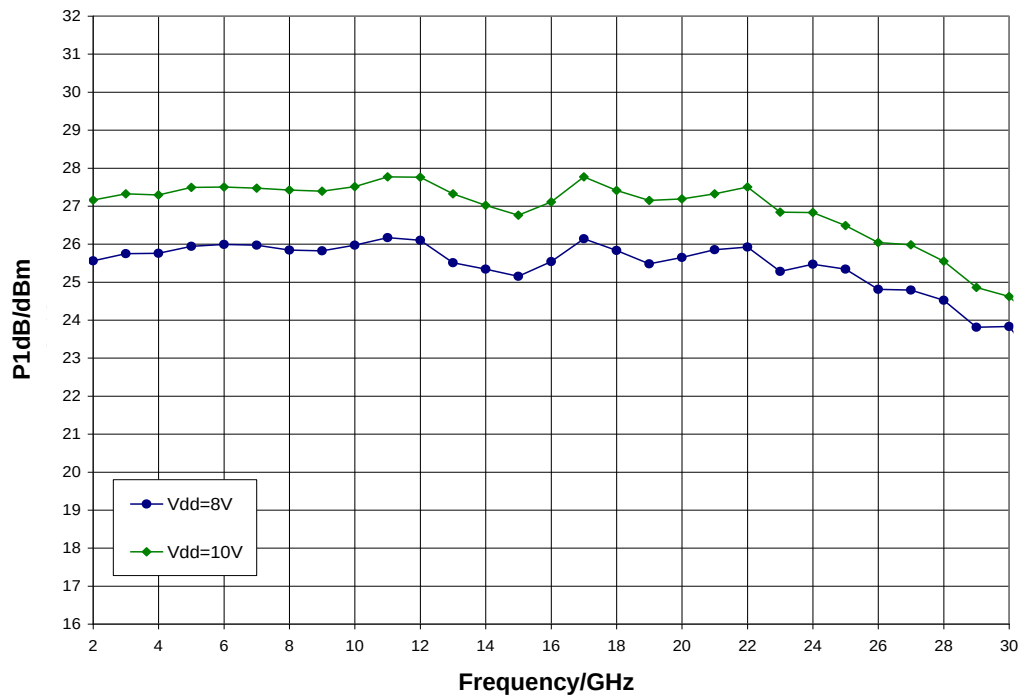
P1dB vs. V_{dd} , V_{gg2} = 3.5\text{ V} , I_{dd} = 250\text{ mA} , T_A = 25^\circ\text{C}
