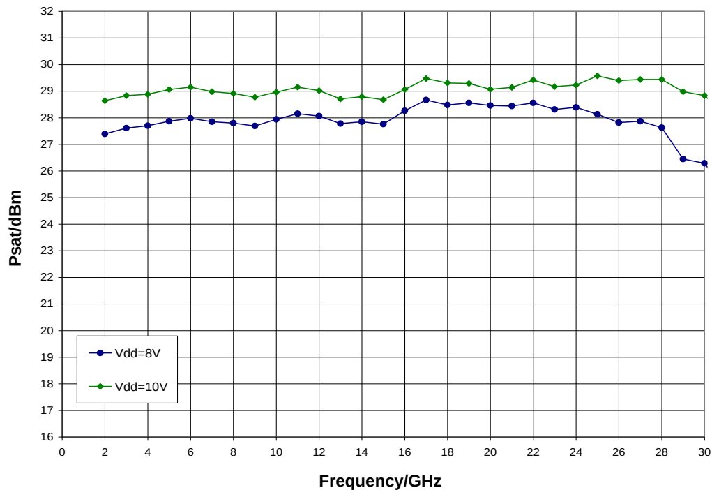
Psat vs. V_{dd} , V_{gg2} = 3.5\text{ V} , I_{dd} = 250\text{ mA} , T_A = 25^\circ\text{C}
