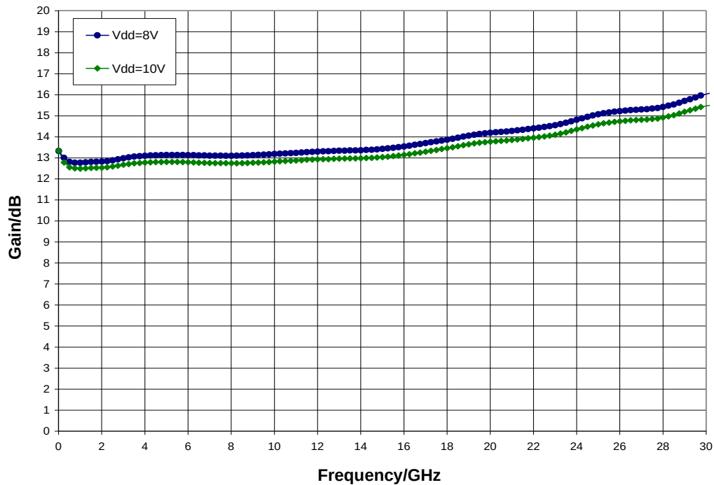
Gain vs. V_{dd} , V_{gg2} = 3.5\text{ V} , I_{dd} = 250\text{ mA} , T_A = 25^\circ\text{C}
