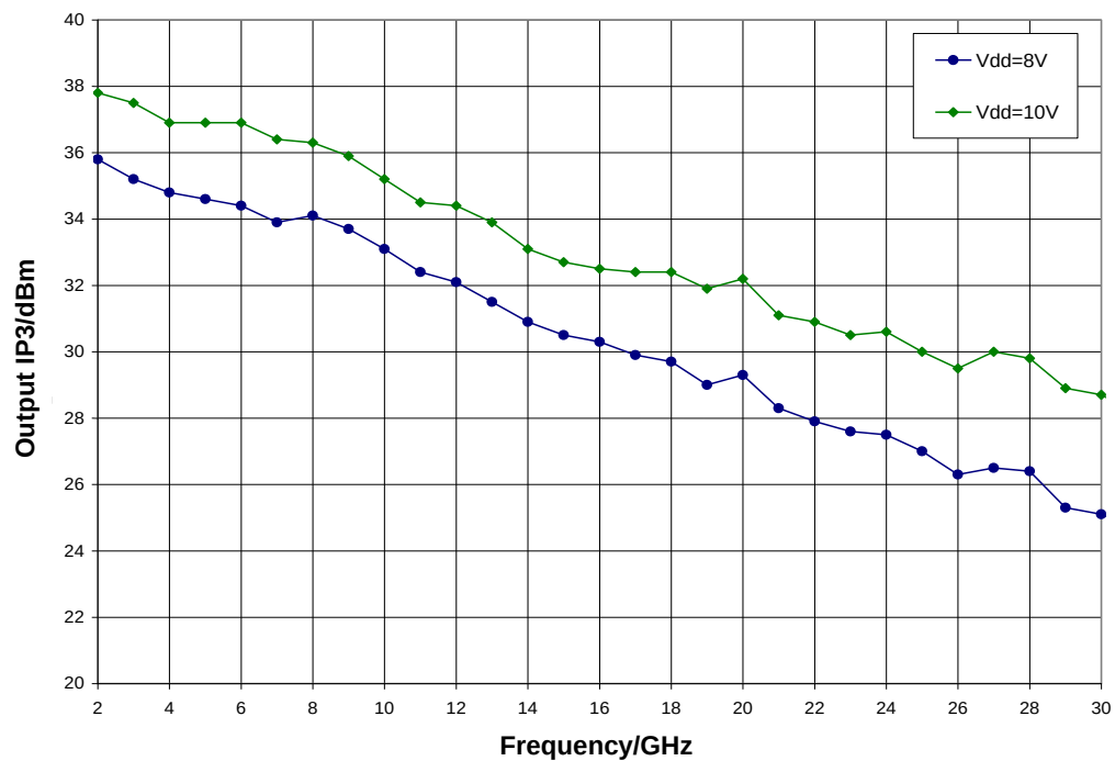
Output IP3 vs. V_{dd} , V_{gg2} = 3.5\text{ V} , I_{dd} = 250\text{ mA} , T_A = 25^\circ\text{C}
