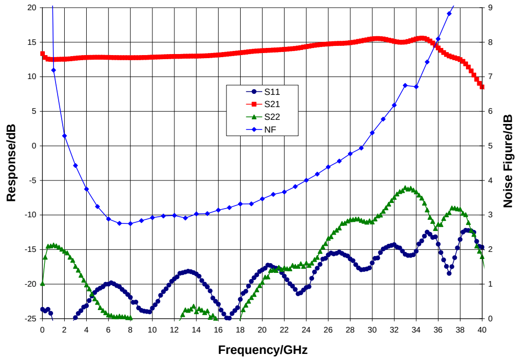
Broadband Performance, V_{dd} = 10\text{ V} , V_{gg2} = 3.5\text{ V} , I_{dd} = 250\text{ mA} , T_A = 25^\circ\text{C}
