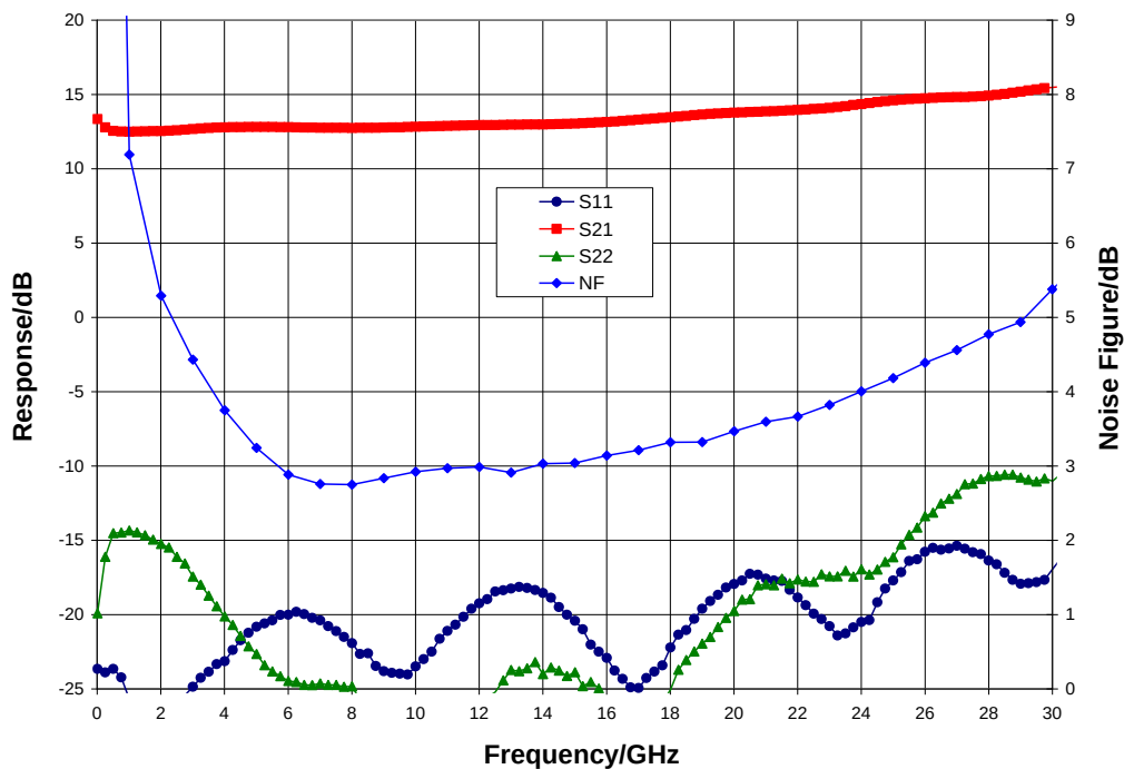
Narrow-band Performance, V_{dd} = 10\text{ V} , V_{gg2} = 3.5\text{ V} , I_{dd} = 250\text{ mA} , T_A = 25^\circ\text{C}
