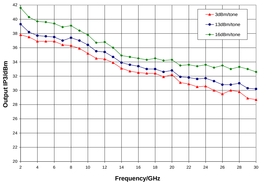
Output IP3 vs. Output Power, V_{dd} = 10\text{ V} , V_{gg2} = 3.5\text{ V} , I_{dd} = 250\text{ mA} , T_A = 25^\circ\text{ C}
