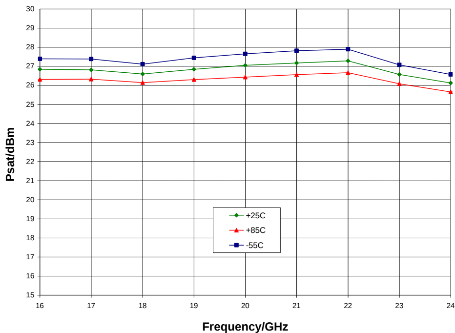
Psat vs. Temperature, V_{dd} = 5\text{ V}
