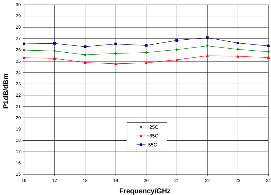
P1dB vs. Temperature, V_{dd} = 5\text{ V}
