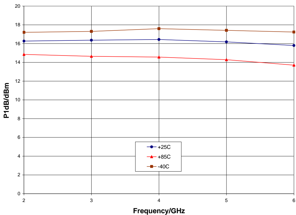
P1dB vs. Temperature, V_{dd} = 3\text{ V} , V_{gg} = 1.5\text{ V}
