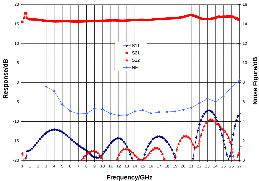
Narrow-band Performance, V_{dd} = 5.0 V, V_{gg} = 3.0 V, I_{dd} = 74 mA, T_A = 25 °C
