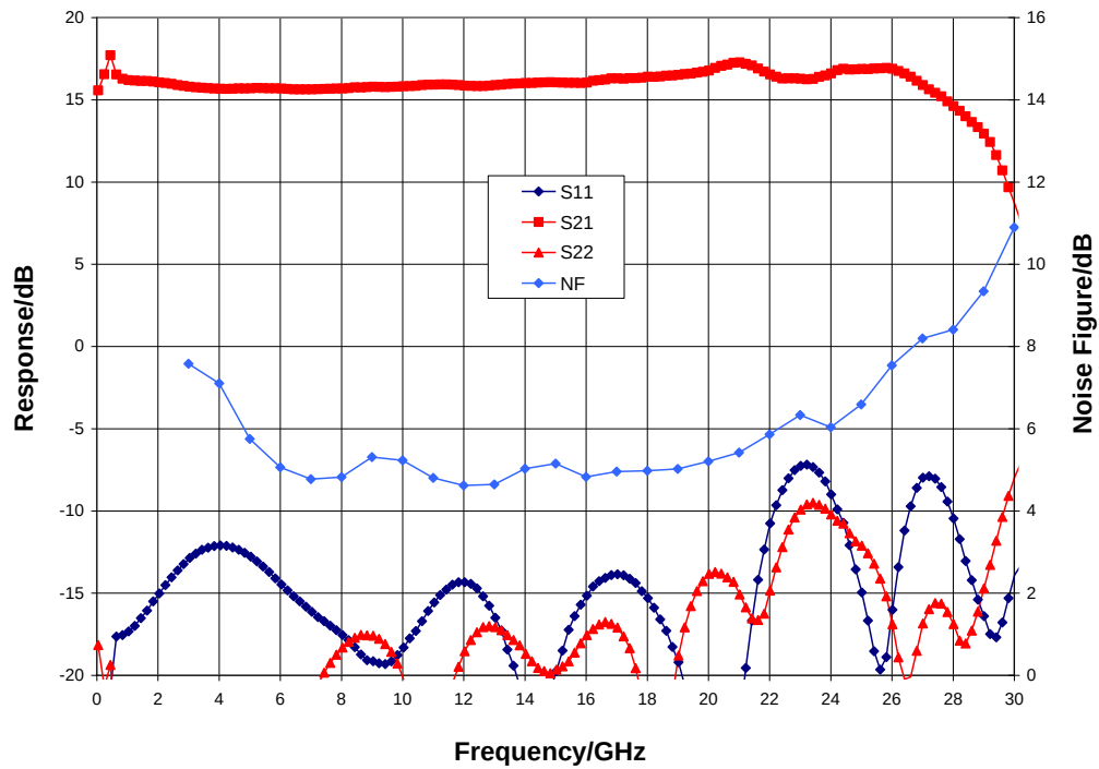
Broadband Performance, V_{dd} = 5.0 V, V_{gg} = 3.0 V, I_{dd} = 74 mA, T_A = 25 °C
