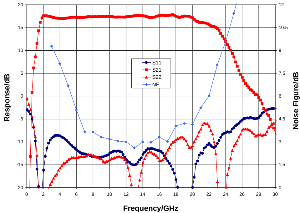
Broadband Performance, V_{dd} = 5.0 V, V_{gg} = 3.0 V, I_{dd} = 74 mA, T_A = 25^\circ C
