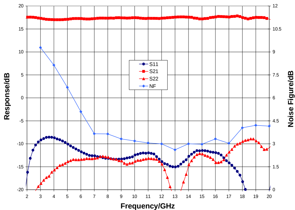
Narrow-band Performance, V_{dd} = 5.0 V, V_{gg} = 3.0 V, I_{dd} = 74 mA, T_A = 25^\circ C
