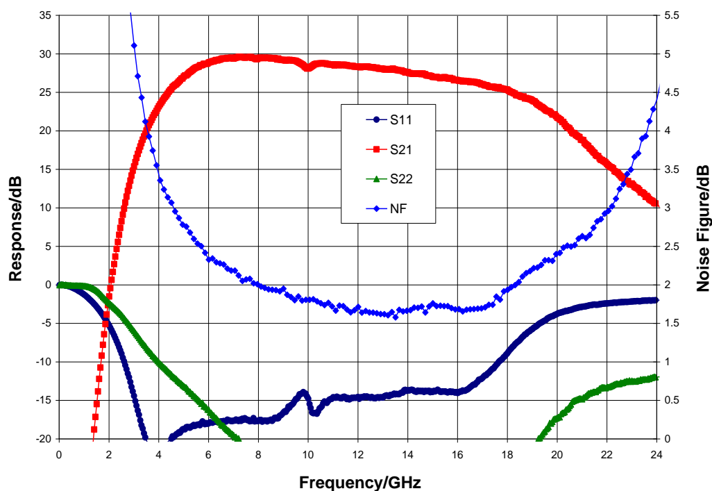
Broadband Performance, V_{dd} = 3.0\text{ V} , I_{dd} = 63\text{ mA} , T_A = 25\text{ }^{\circ}\text{C}
