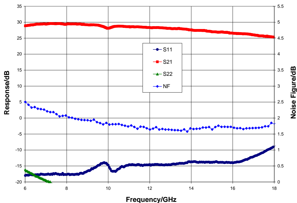
Narrow-band Performance, V_{dd} = 3.0\text{ V} , I_{dd} = 63\text{ mA} , T_A = 25\text{ }^{\circ}\text{C}
