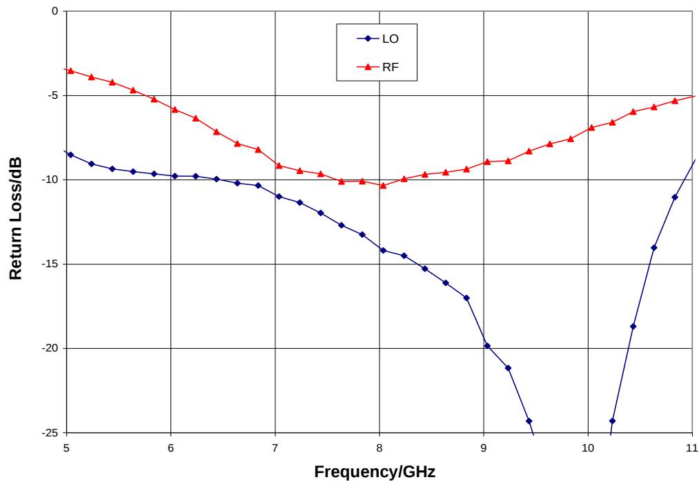
Return Loss, LO = +21 dBm
