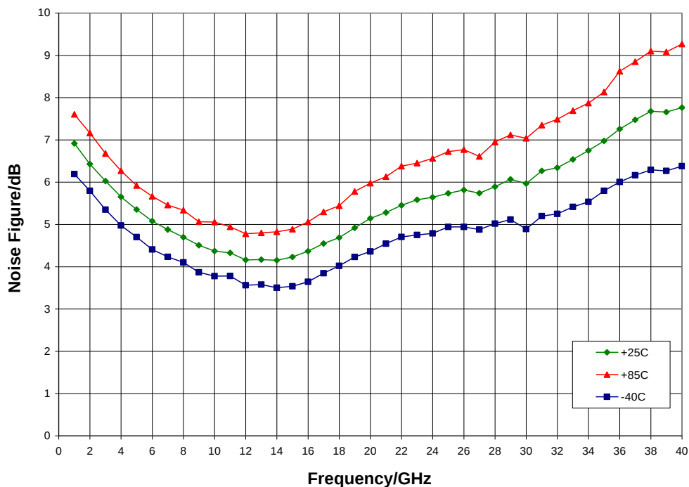
Noise Figure vs. Temperature, V_{dd} = 8 V
