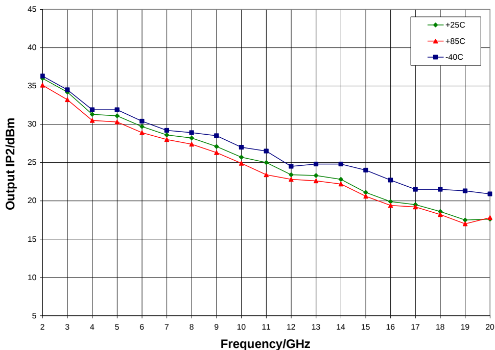
Output IP2 vs. Temperature, V_{dd} = 8 V
