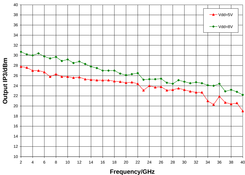
Output IP3 vs. V_{dd} , I_{dd} = 100 mA, T_A = 25^\circ\text{C}
