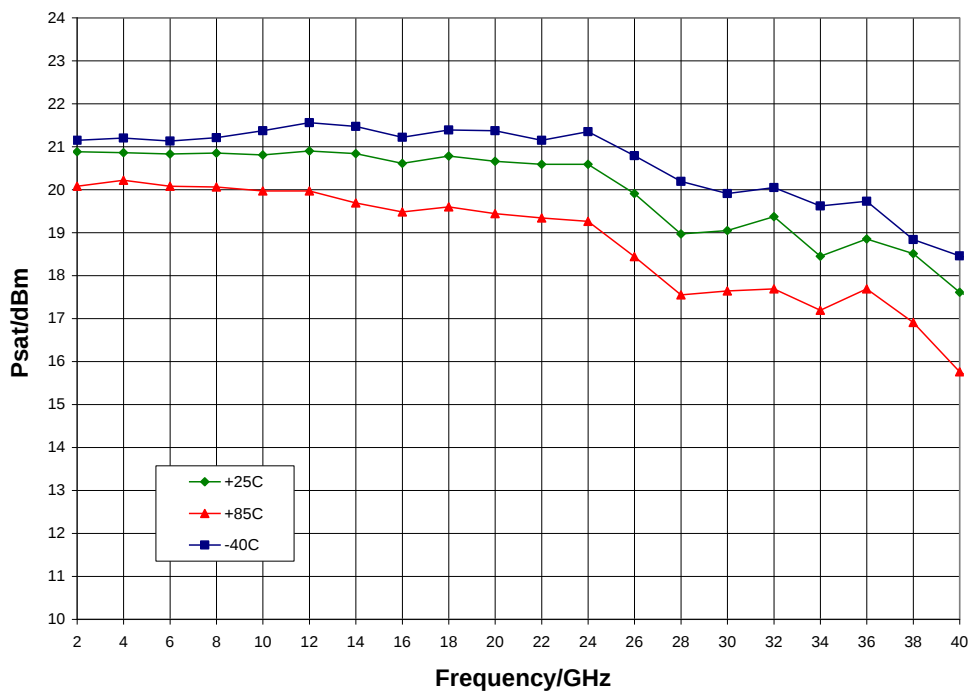
Psat vs. Temperature, V_{dd} = 8\text{ V}
