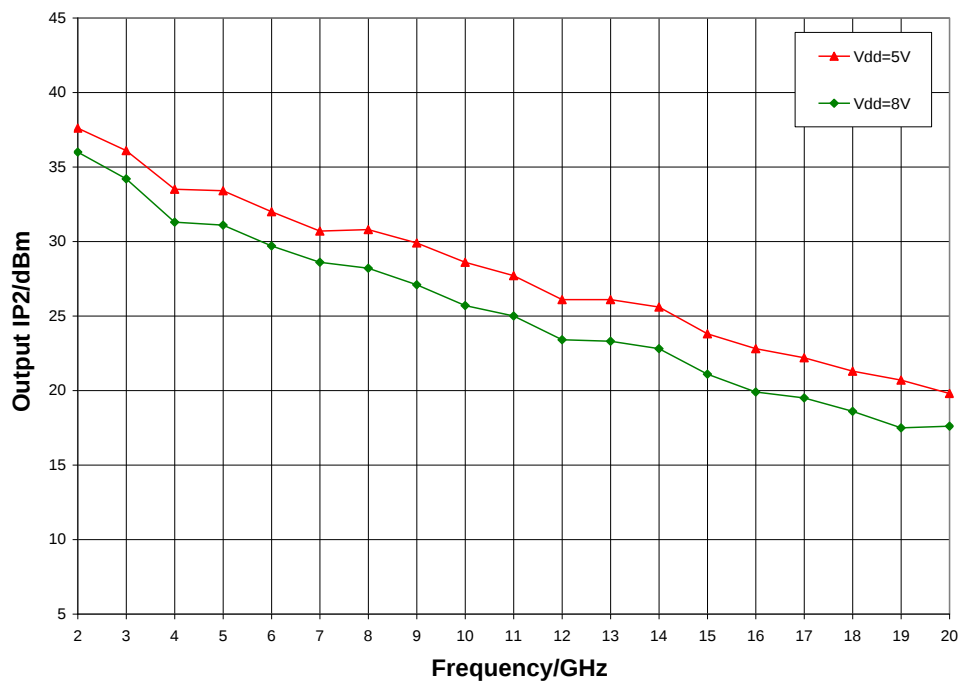
Output IP2 vs. V_{dd} , I_{dd} = 100 mA, T_A = 25^\circ C
