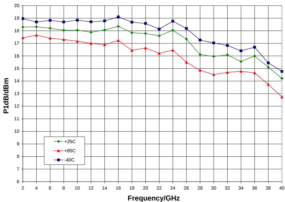
P1dB vs. Temperature, V_{dd} = 8 V
