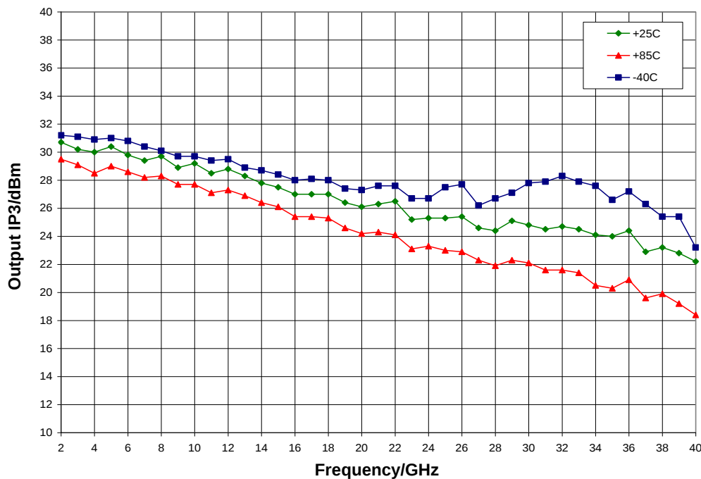
Output IP3 vs. Temperature, V_{dd} = 8\text{ V}
