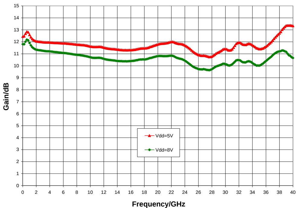
Gain vs. V_{dd} , I_{dd} = 100 mA, T_A = 25^\circ\text{C}
