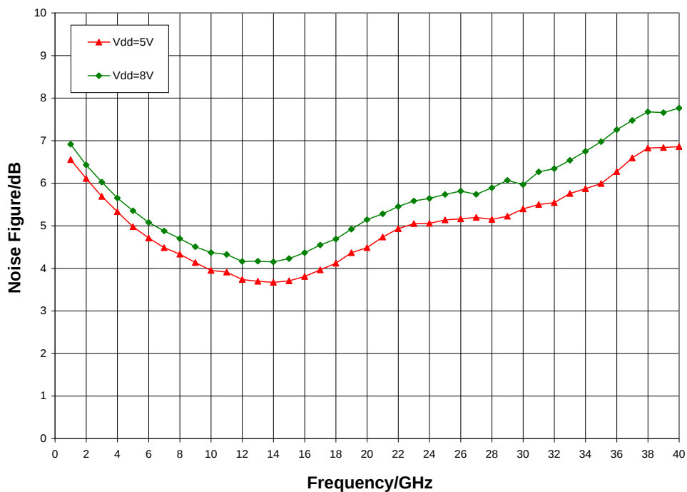
Noise Figure vs. V_{dd} , I_{dd} = 100 mA, T_A = 25^\circ C
