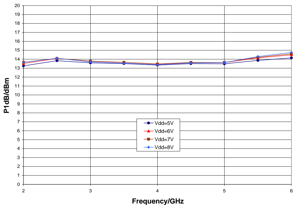
P1dB vs. Supply Voltage, T_A = 25\text{ °C}
