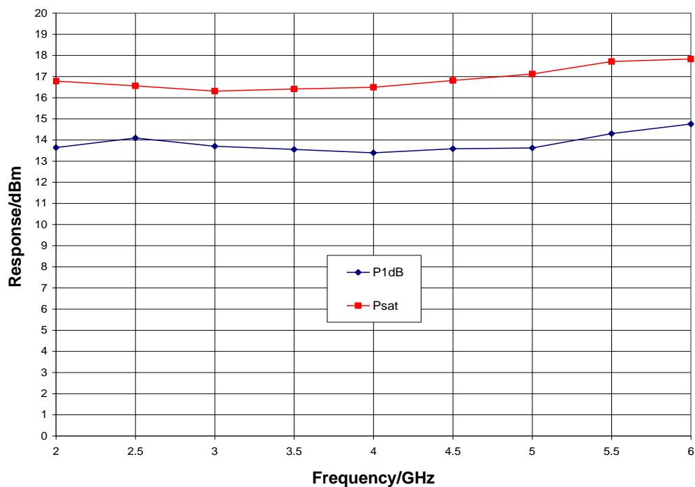
Output Power, V_{dd} = 8.0 \text{ V} , T_A = 25 \text{ }^{\circ}\text{C}
