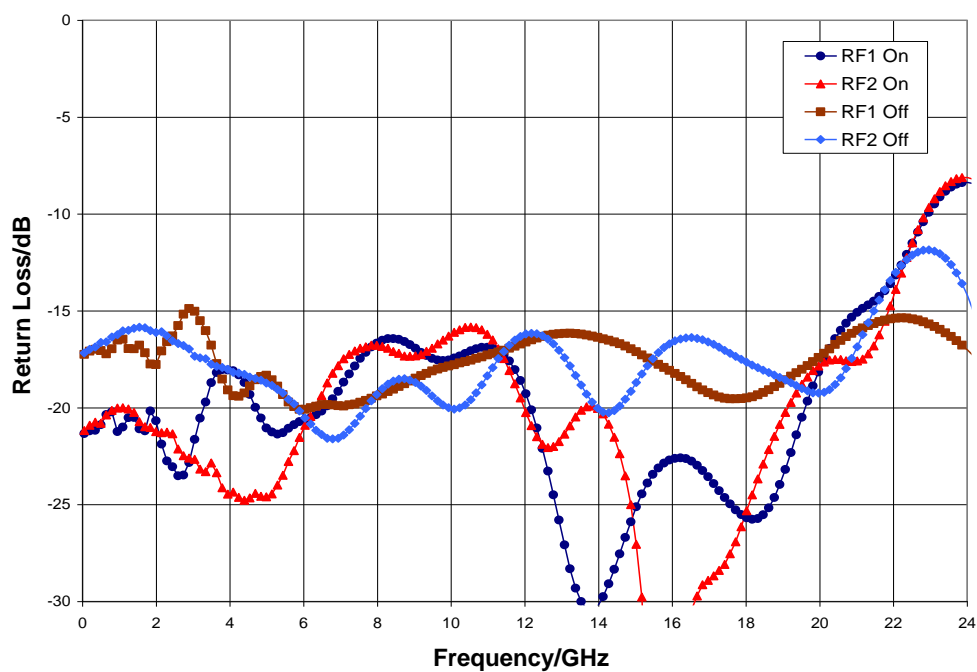
Return Loss
