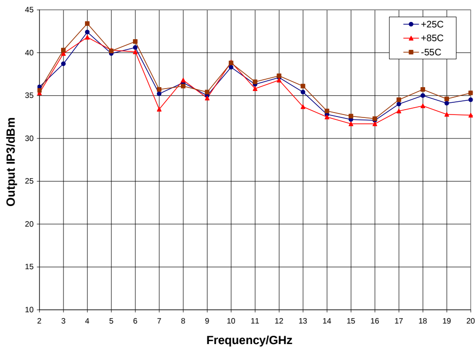
Output IP3 vs. Temperature, V_{dd} = 10\text{ V} , V_{gg1} = -0.55\text{ V} , V_{gg2} = 5\text{ V}
