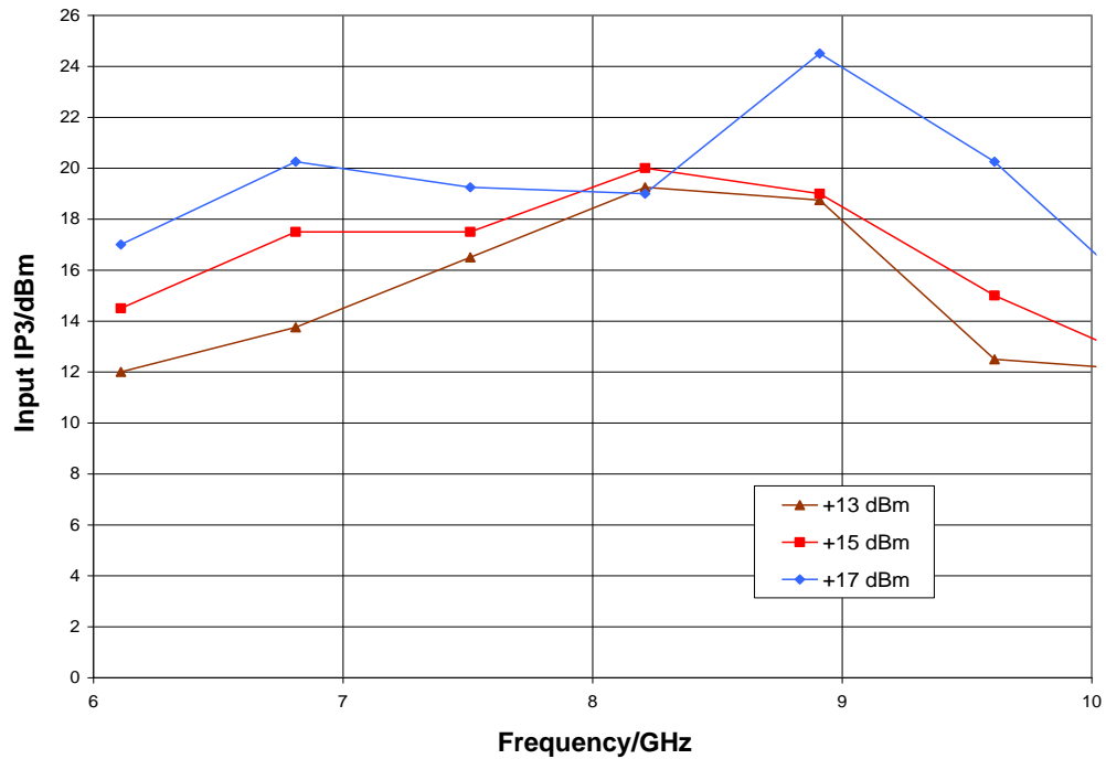
Upconverter Performance, Input IP3 vs. LO Drive, IF = 500 MHz
