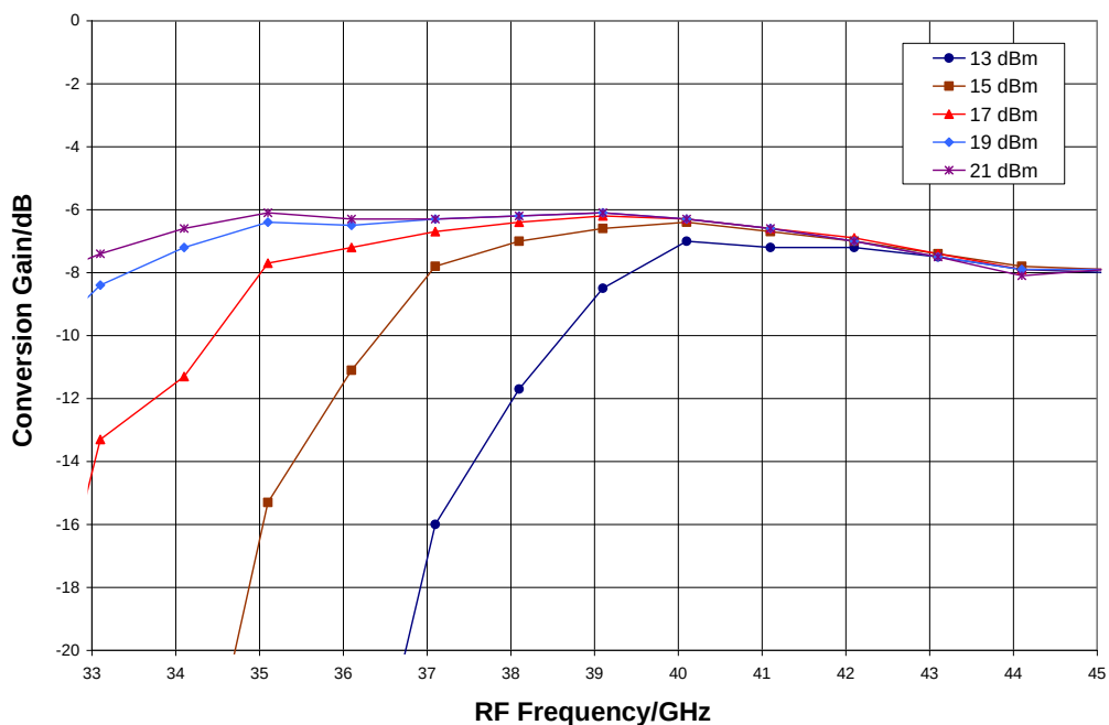
Conversion Gain vs. LO Drive, IF = 5 GHz USB
