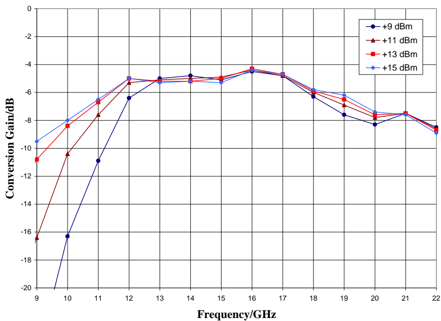
Upconverter Performance, Conversion Gain vs. LO Drive, IF Input = 100 MHz
