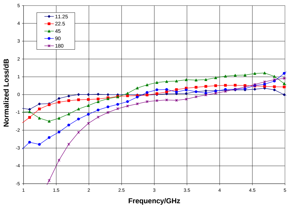
Normalized Loss, Major States, V_{ee} = -3.0\text{ V}
