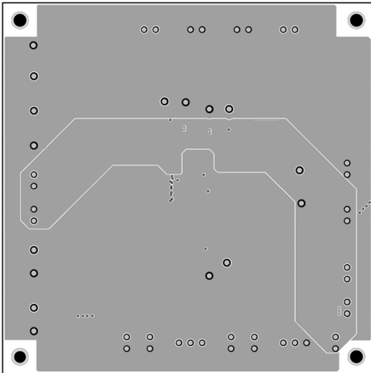
Figure 7 – Layout Layer 2
