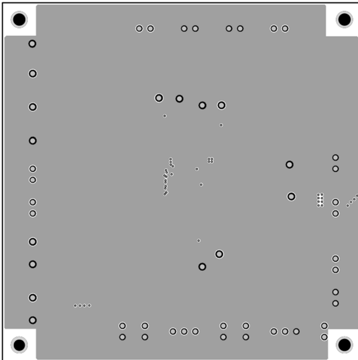
Figure 7 – Layout Layer 3
