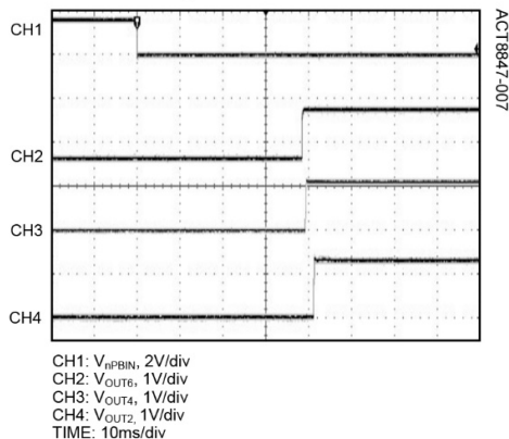
Startup of nPBIN, OUT6/4/2
