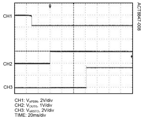
Startup of nPBIN, OUT6, nRSTO
