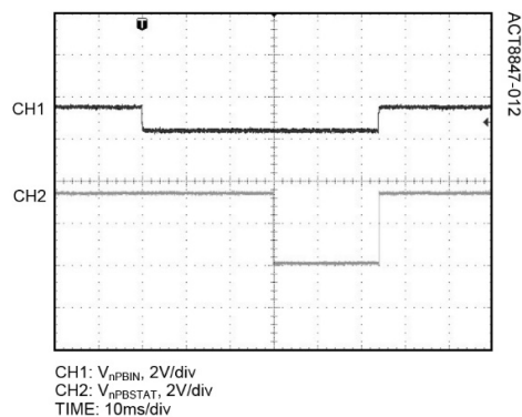
nPBIN and nPBSTAT
