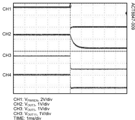
Sleep of PWREN, OUT3/5/11
