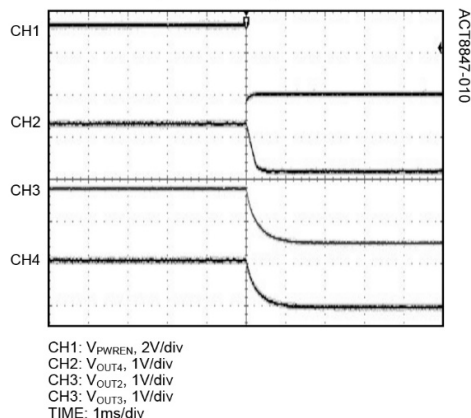
Sleep of PWREN, OUT4/2/3
