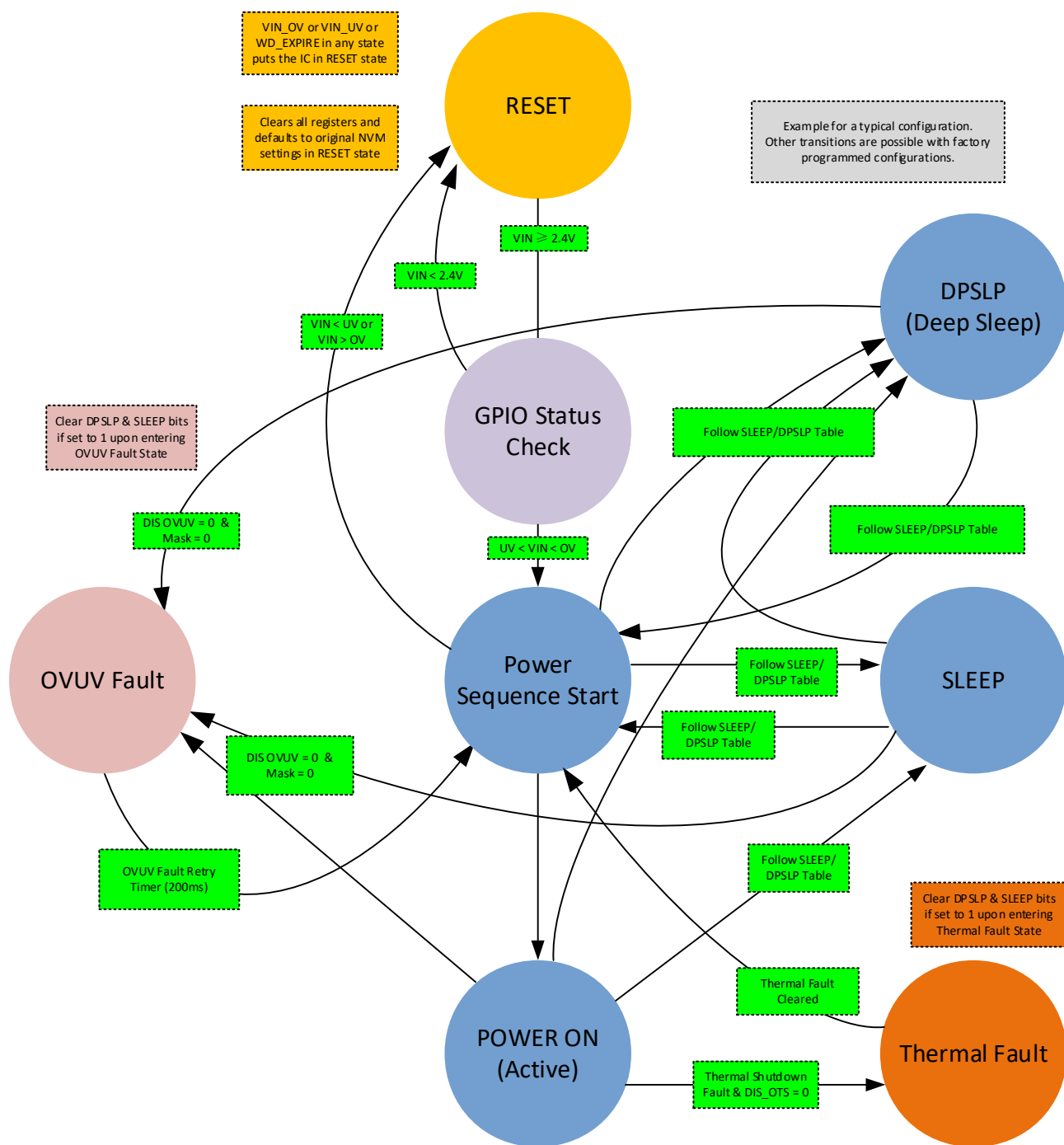
Figure 6: State Machine
