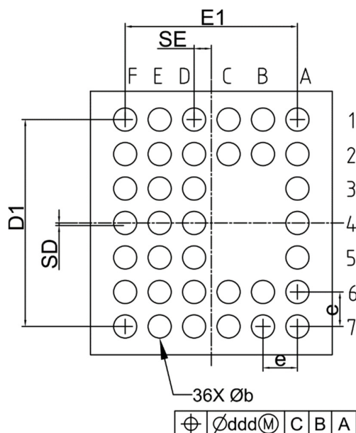
Bottom View
