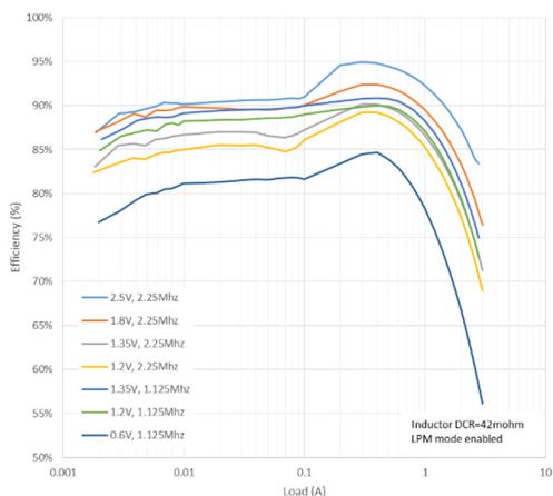
BUCK2 Efficiency, Vin=3.3V
