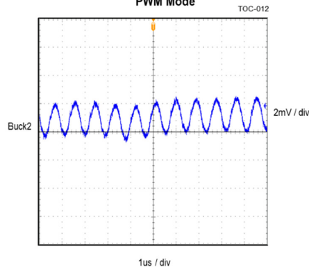
Buck2 Voltage Ripple PWM Mode
