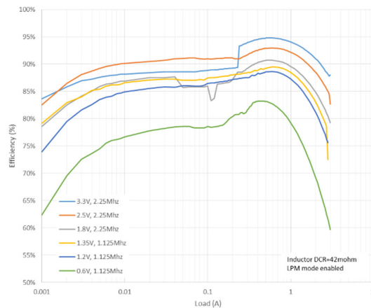
BUCK2 Efficiency, Vin=5.0V
