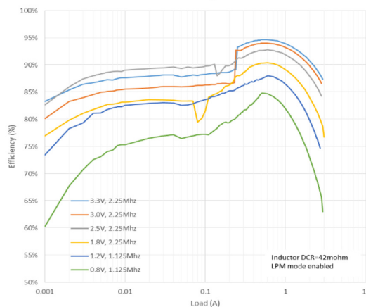
BUCK3 Efficiency, Vin=5.0V
