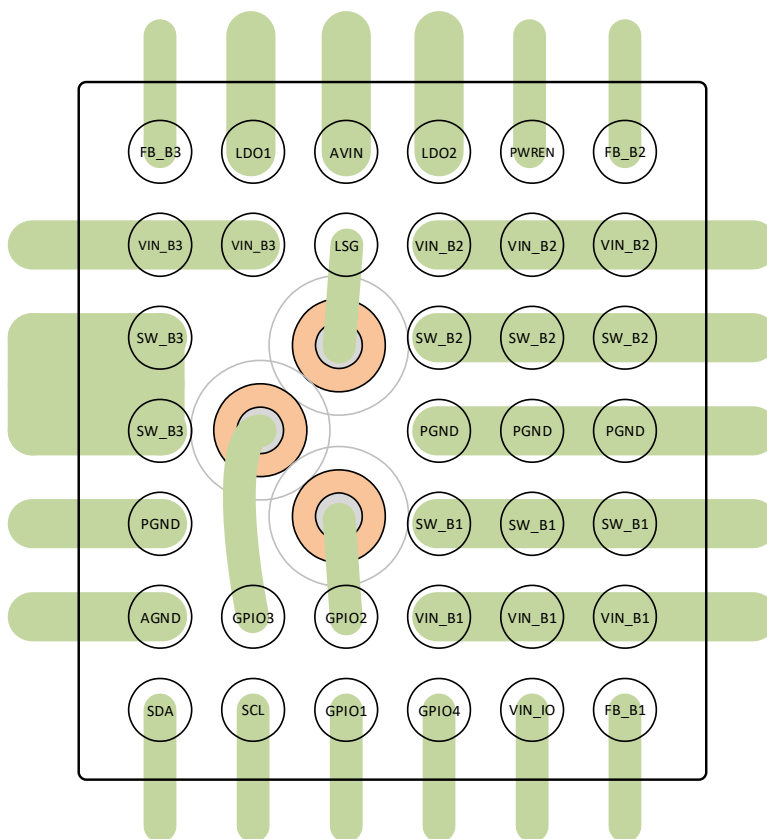
Figure 4: Recommended Routing
