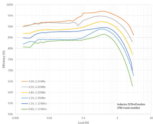
BUCK3 Efficiency, Vin=3.3V
