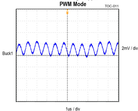
Buck1 Voltage Ripple PWM Mode
