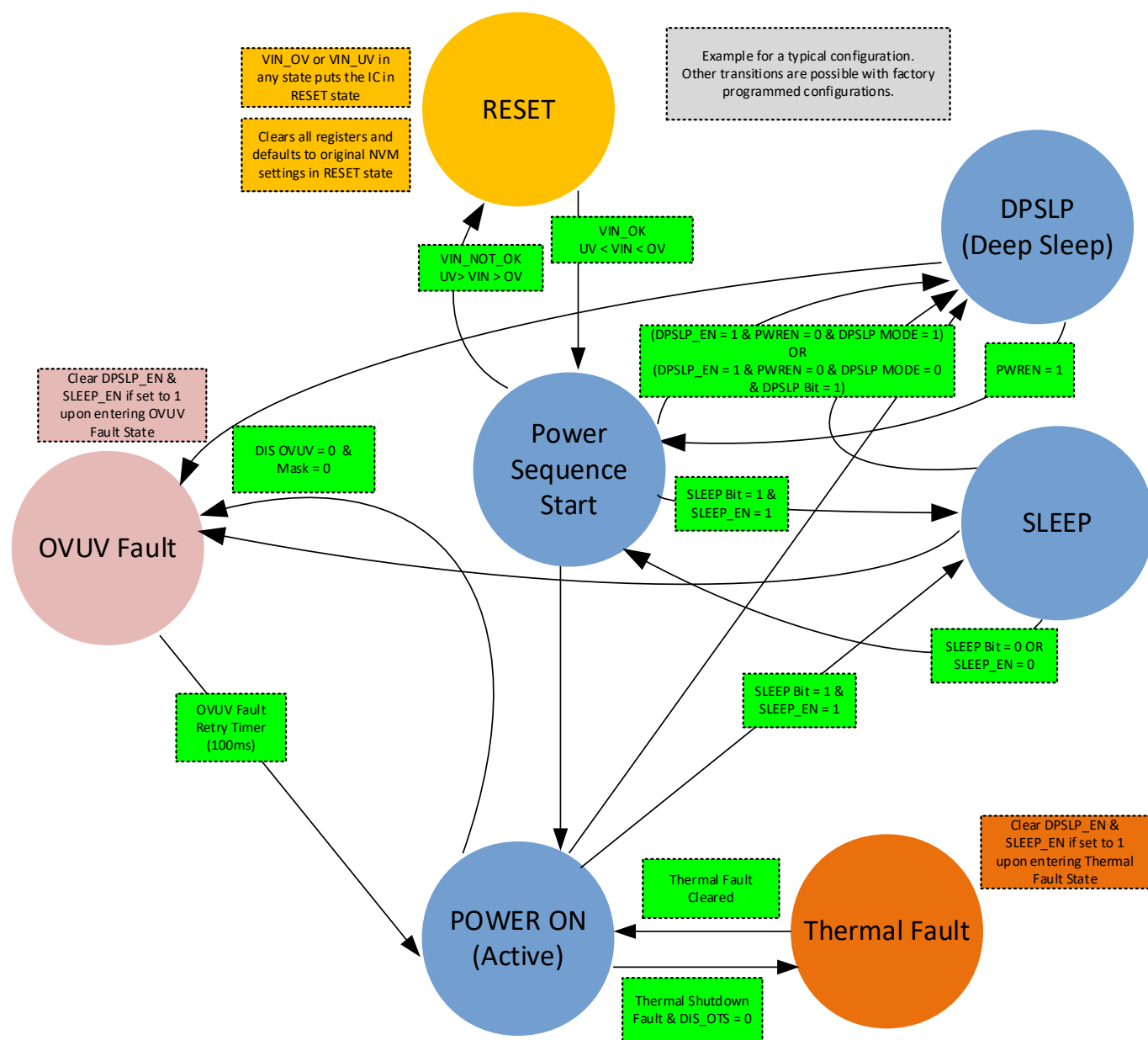
Figure 3: PWREN State Machine
