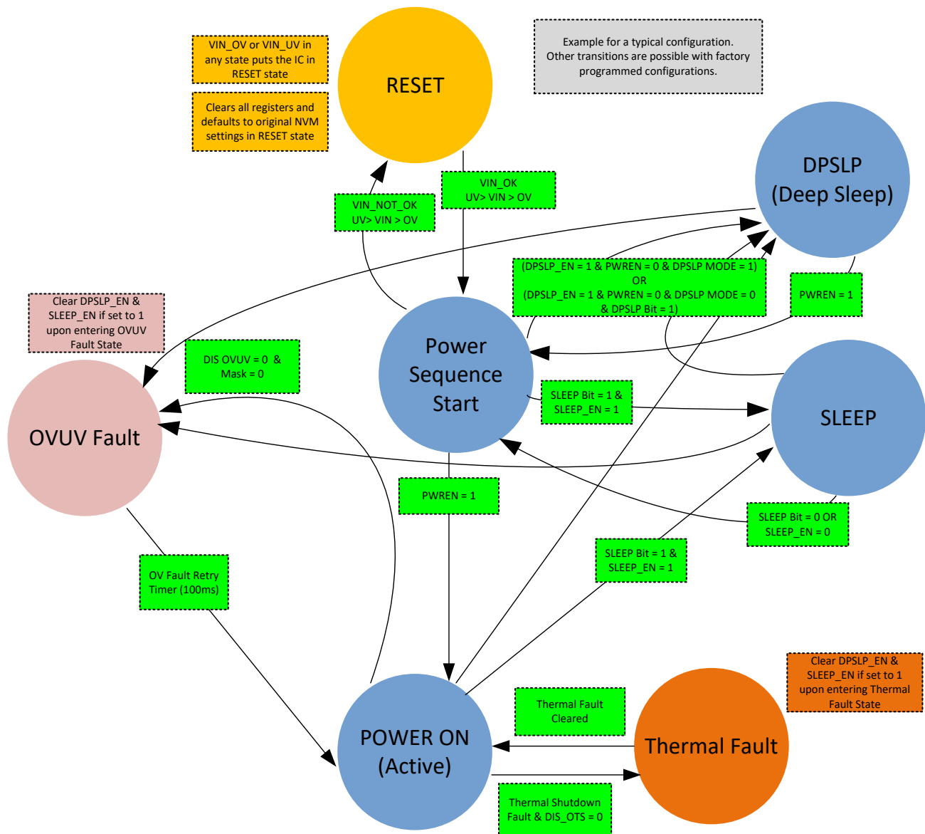
Figure 5: ACT81461 State Diagram
