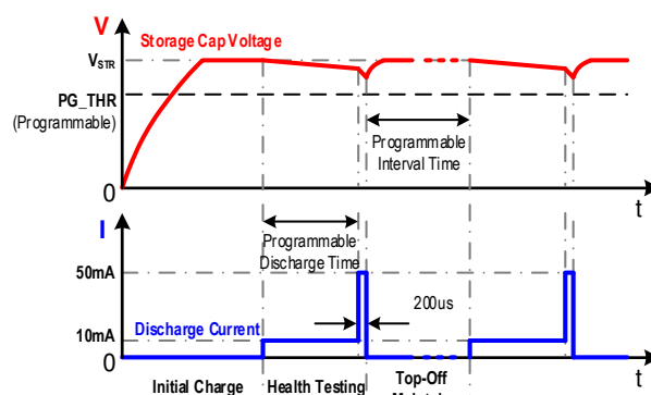
Figure 6: Storage Voltage at Different Stages
