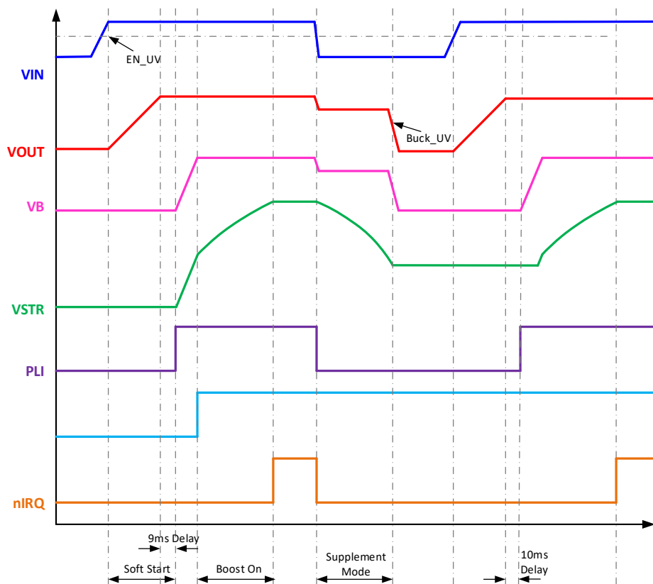
Figure 4: Operation State
