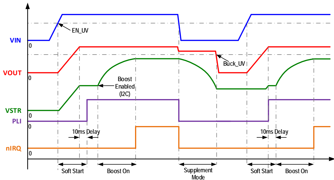
Figure 4: Operation states
