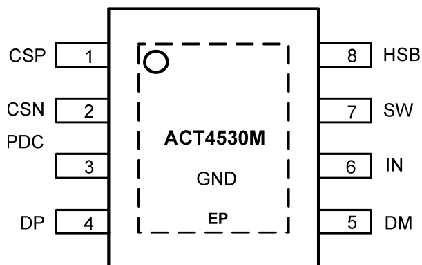
SOP-8EP
