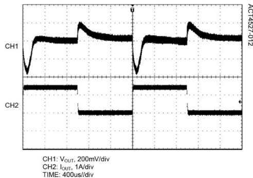
Load Transient (1A-2.4A-1A) V_{in}=12.6\text{V} , V_{out}=12\text{V}
