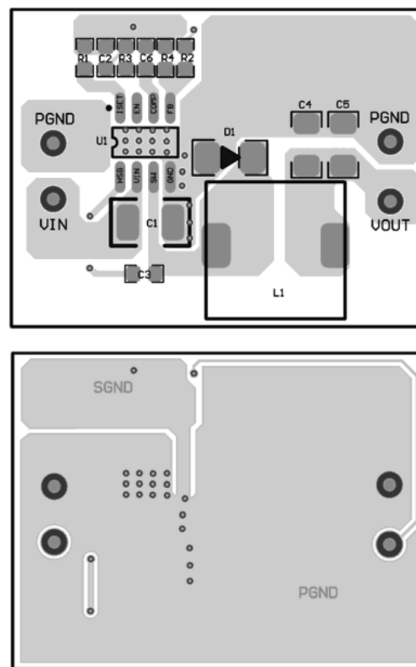
Figure 7: PCB Layout
