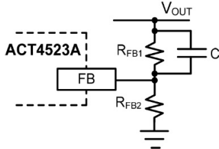
Figure 1: Output Voltage Setting
