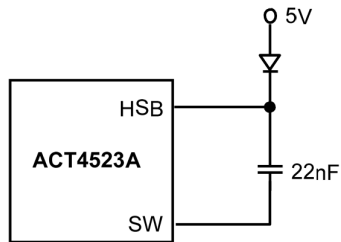
Figure 3: External High Voltage Bias Diode
