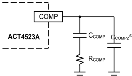
Figure 4: Stability Compensation
