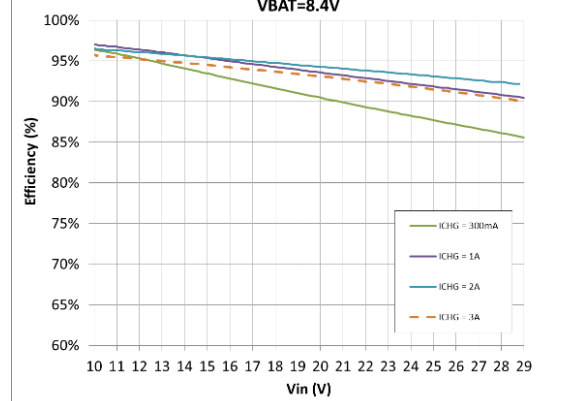
Efficiency Charger VBAT=8.4V
