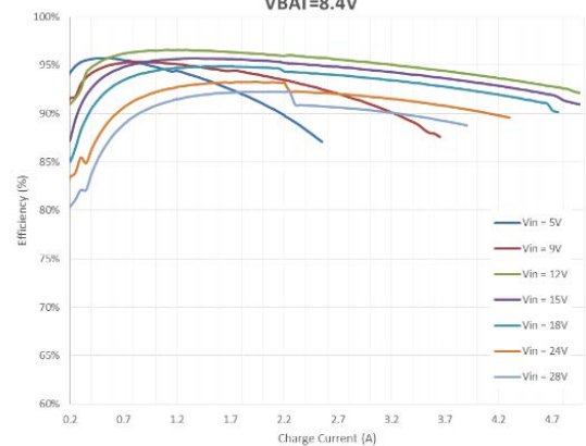
Efficiency - Charger VBAT=8.4V
