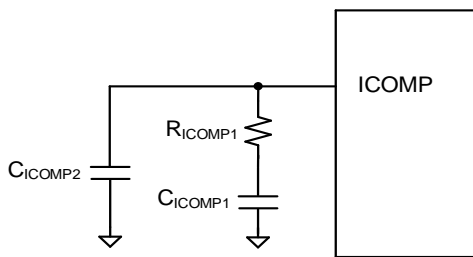
Figure 16: OTG Compensation
