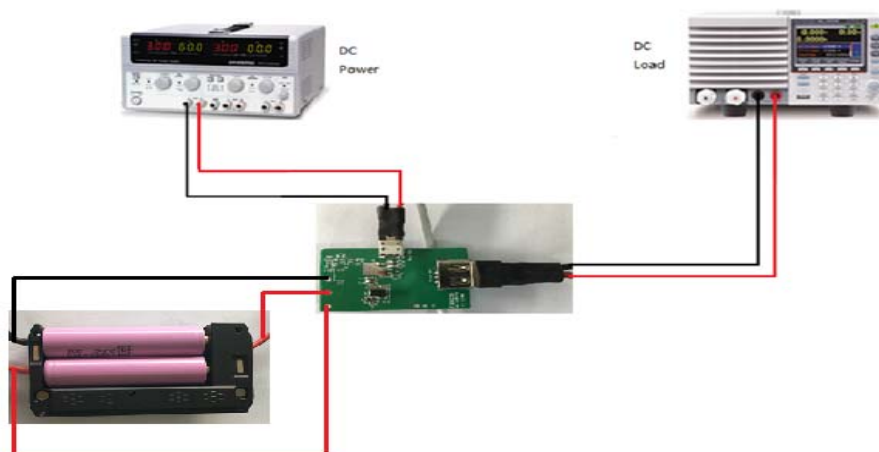
EVK Setup
