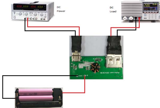
Figure 3 – EVK Setup
