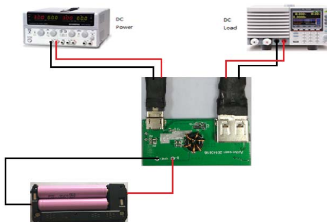
Figure 3 – EVK Setup
