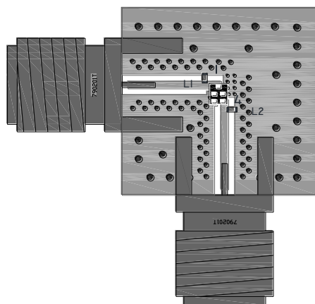
Figure 2a. 885128 Evaluation Board Image
