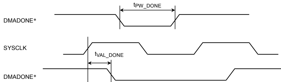
Figure 21.5.9 Timing Diagram: DMA Interface
