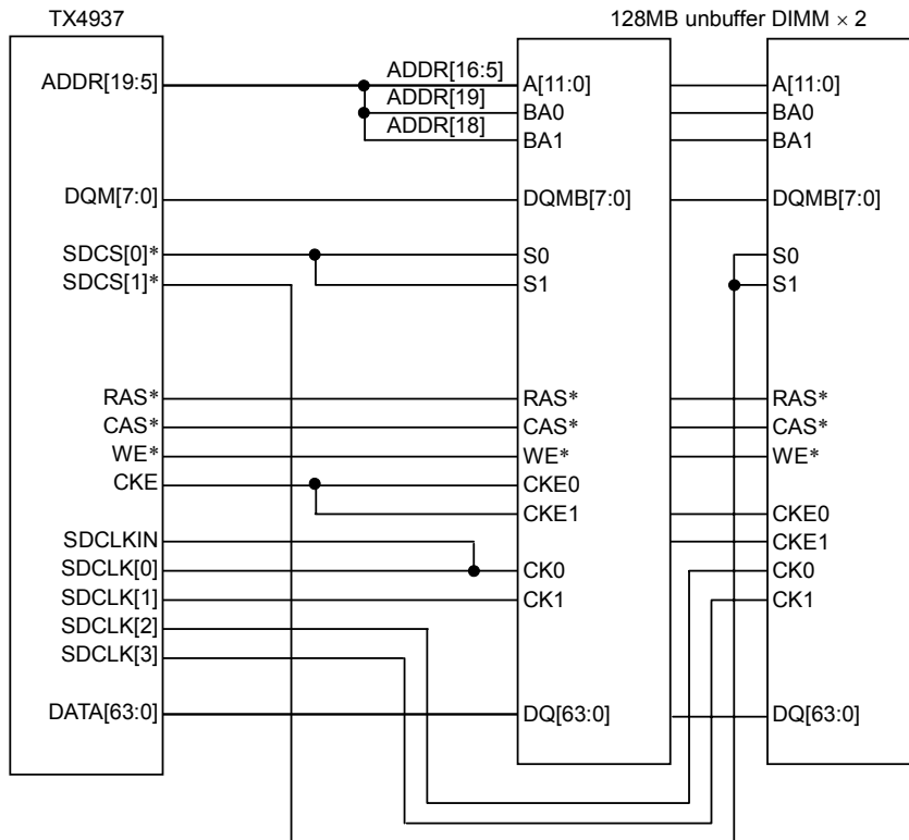
Figure 9.6.2 168-pin DIMM Connection Example
