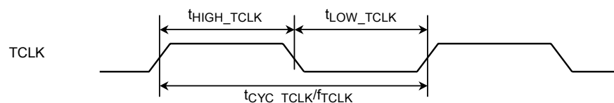
Figure 21.5.12 Timing Diagram: Timer Interface
