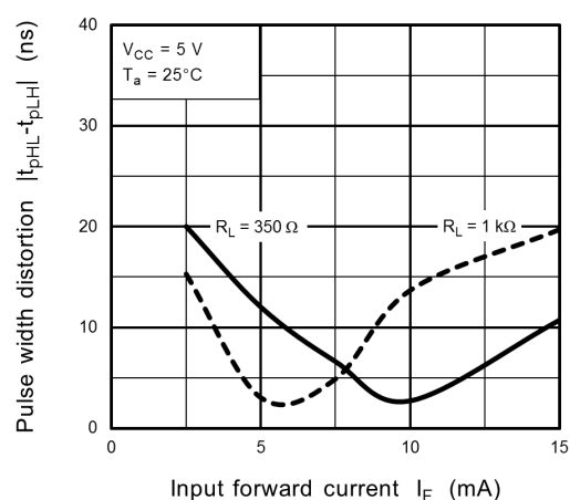
Fig. 11.2.24 |t_{pHL} - t_{pLH}| - I_F
