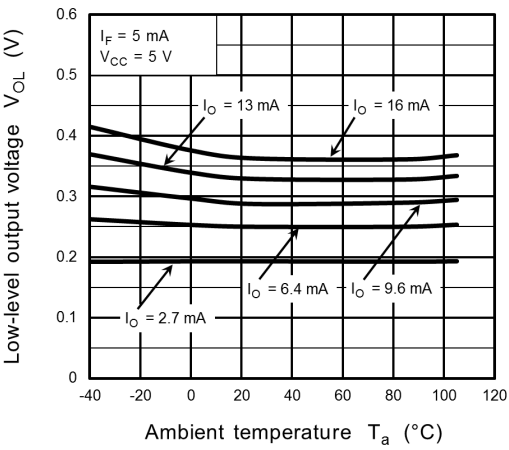
Fig. 11.2.6 V_{OL} - T_a
