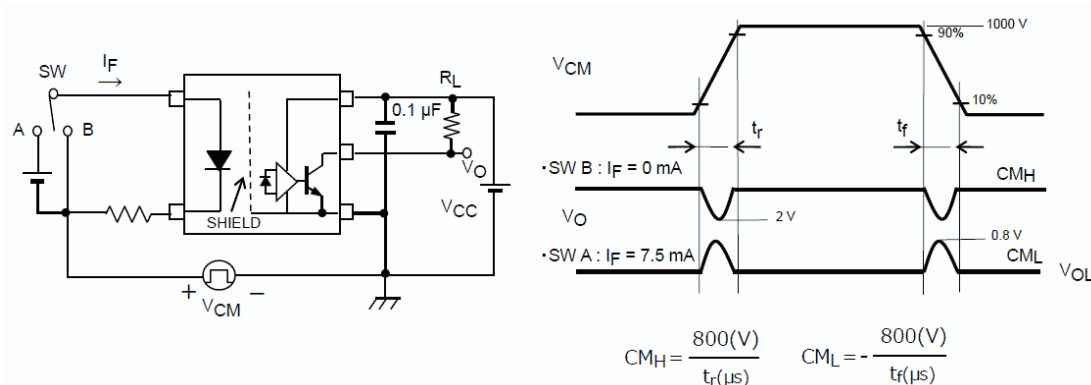
Fig. 11.1.6 Common-Mode Transient Immunity Test Circuit and Waveform
