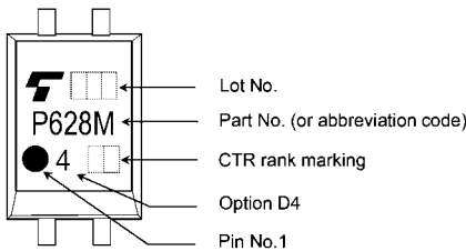
Fig. 15.4 Marking Example of TLP628M (Note 1)
