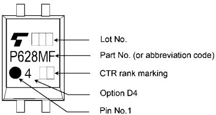
Fig. 15.5 Marking Example TLP628MF (Note 1)
