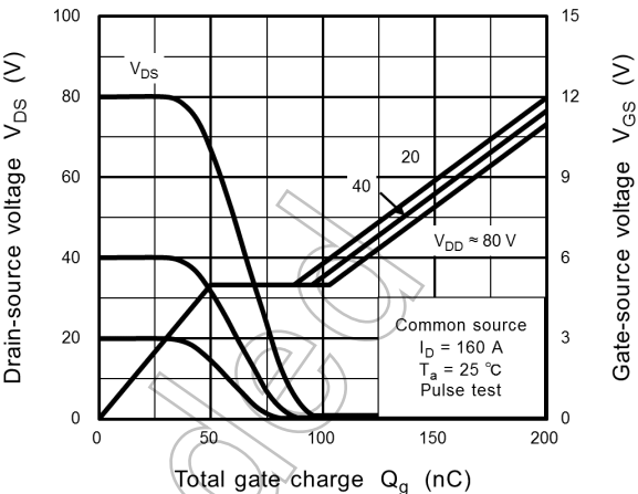
Fig. 9.14 Dynamic Input/Output Characteristics
