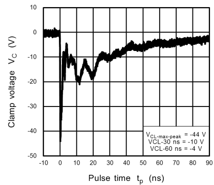
Fig. 10.10.4 IEC61000-4-2 Clamp Waveform -8 kV
