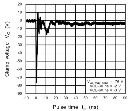
Fig. 10.10.6 ISO10605 Clamp Waveform -8 kV
