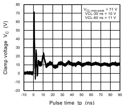
Fig. 10.6.5 ISO10605 Clamp Waveform +8 kV
