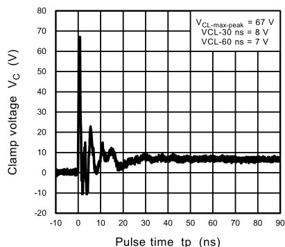
Fig. 10.2.5 ISO10605 Clamp Waveform +8 kV
